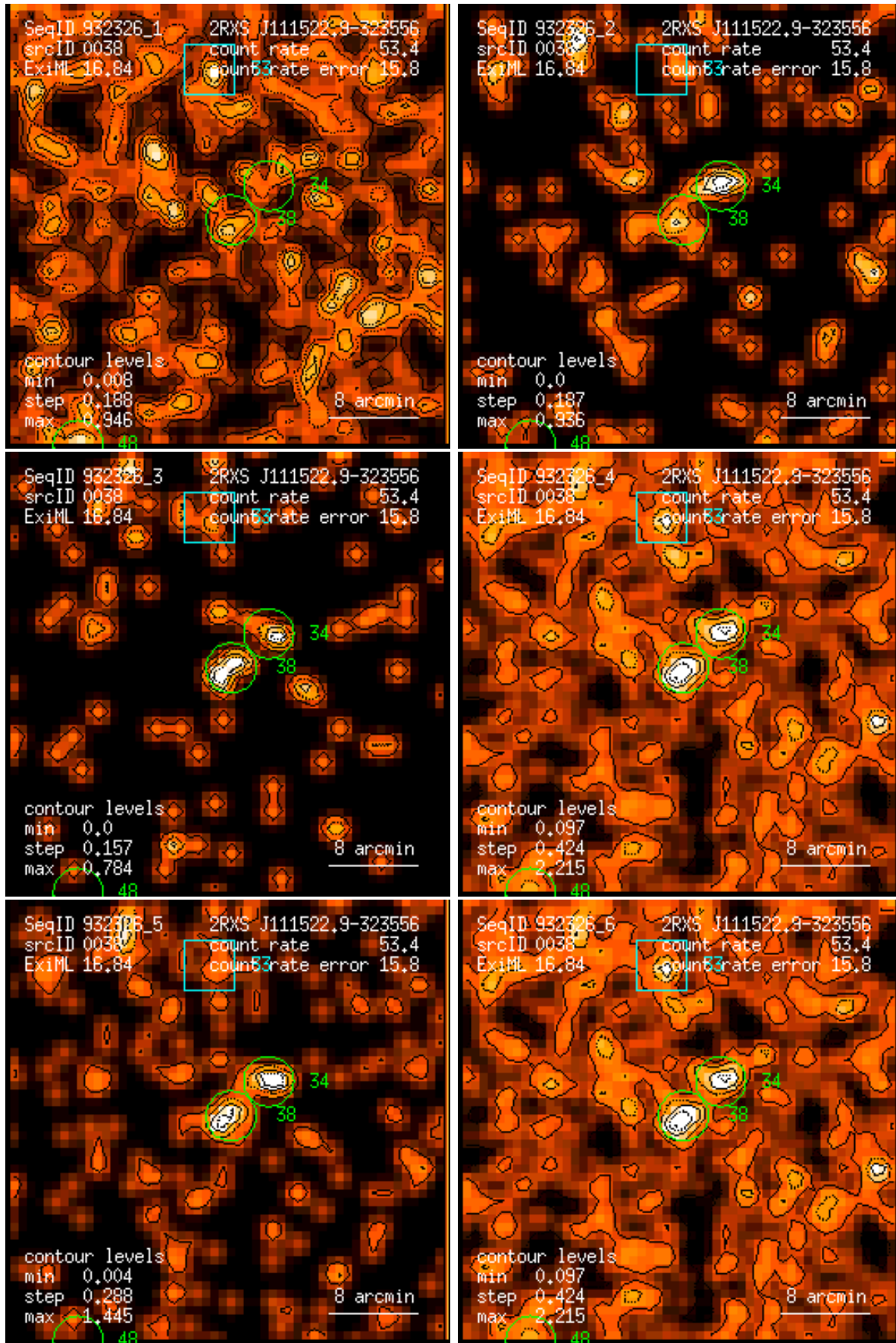
Figure 38: RASS 932326: detection 0038: band rate images, Gaussian filter: (1) PSPC channels 11 – 41, (2) 52 – 90, (3) 91 – 201, (4) 11 – 235, (5) 52 – 201, (6) 11 – 201. Broad band rates in counts/ks. Band rate contour levels in counts/ks/arcmin 2 .
