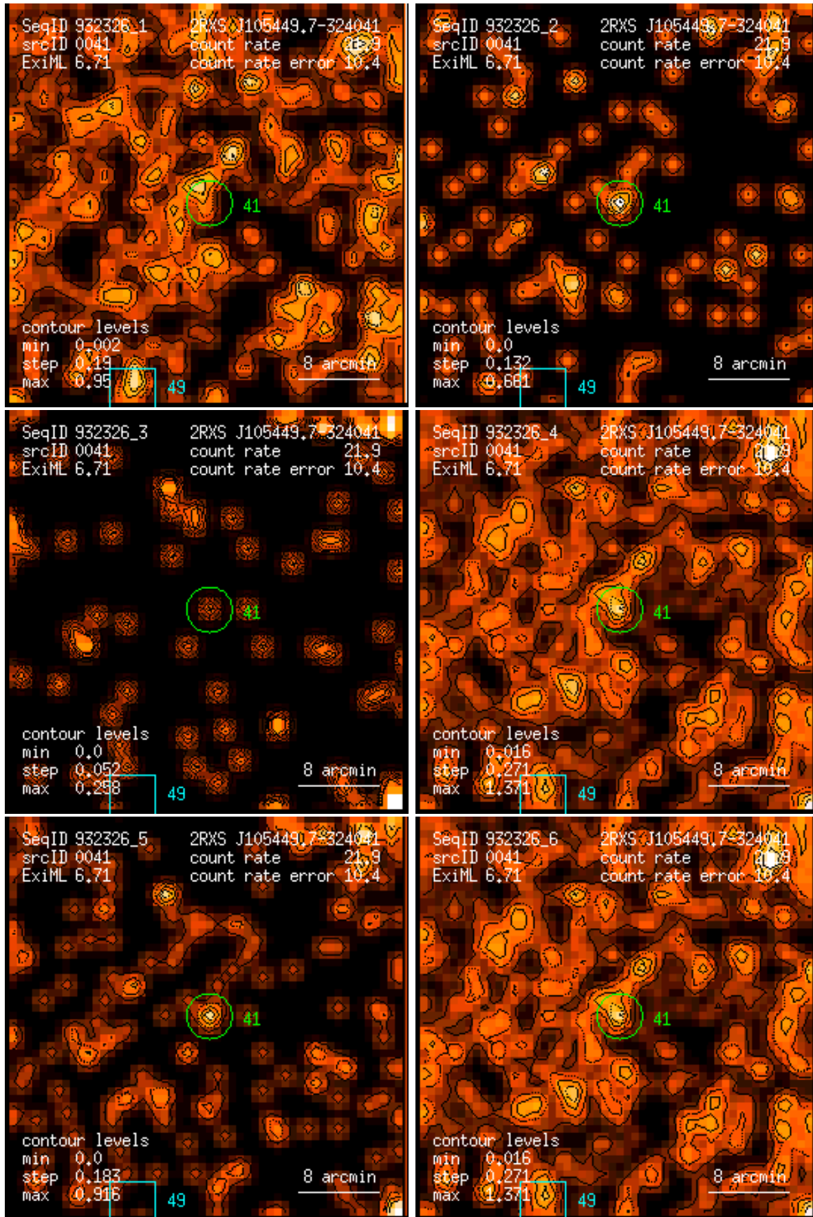
Figure 41: RASS 932326: detection 0041: band rate images, Gaussian filter: (1) PSPC channels 11 – 41, (2) 52 – 90, (3) 91 – 201, (4) 11 – 235, (5) 52 – 201, (6) 11 – 201. Broad band rates in counts/ks. Band rate contour levels in counts/ks/arcmin 2 .
