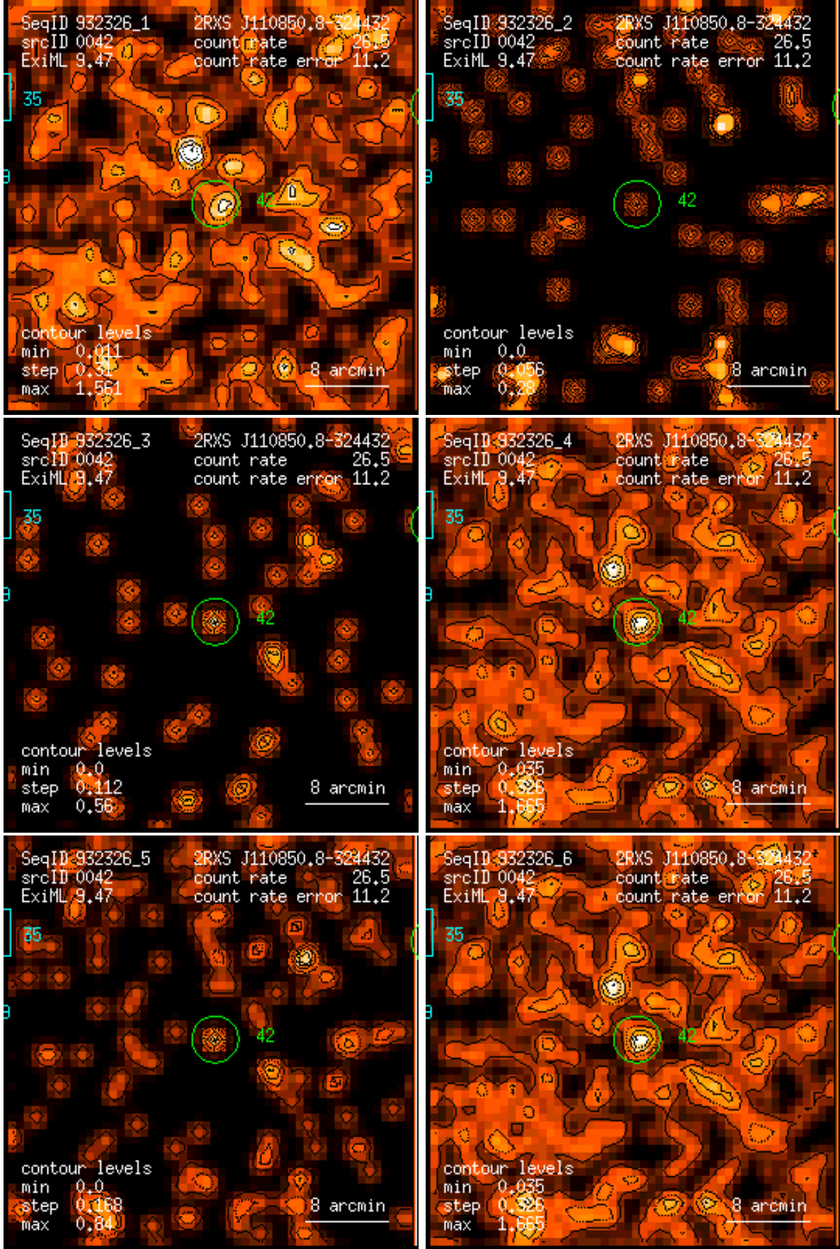
Figure 42: RASS 932326: detection 0042: band rate images, Gaussian filter: (1) PSPC channels 11 – 41, (2) 52 – 90, (3) 91 – 201, (4) 11 – 235, (5) 52 – 201, (6) 11 – 201. Broad band rates in counts/ks. Band rate contour levels in counts/ks/arcmin 2 .
