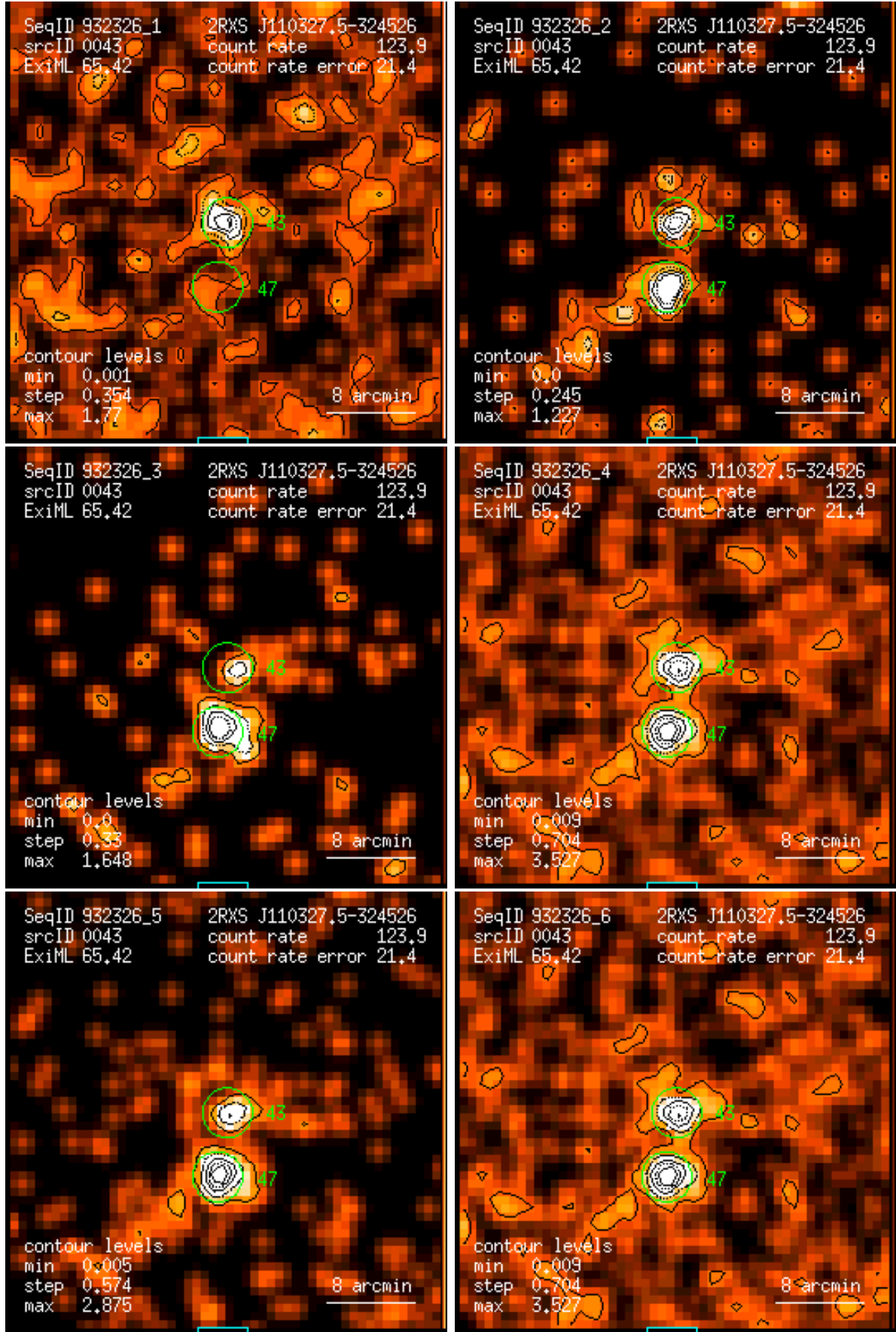
Figure 43: RASS 932326: detection 0043: band rate images, Gaussian filter: (1) PSPC channels 11 – 41, (2) 52 – 90, (3) 91 – 201, (4) 11 – 235, (5) 52 – 201, (6) 11 – 201. Broad band rates in counts/ks. Band rate contour levels in counts/ks/arcmin 2 .
