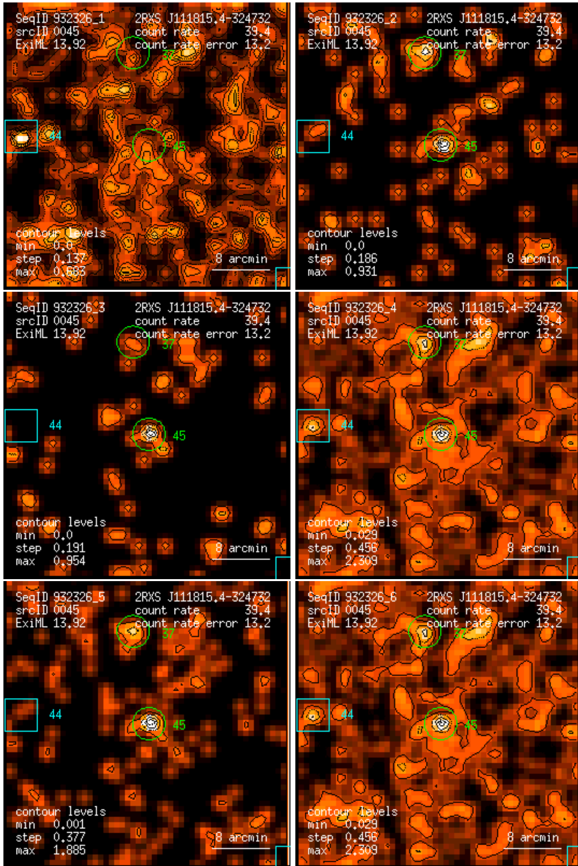
Figure 45: RASS 932326: detection 0045: band rate images, Gaussian filter: (1) PSPC channels 11 – 41, (2) 52 – 90, (3) 91 – 201, (4) 11 – 235, (5) 52 – 201, (6) 11 – 201. Broad band rates in counts/ks. Band rate contour levels in counts/ks/arcmin 2 .
