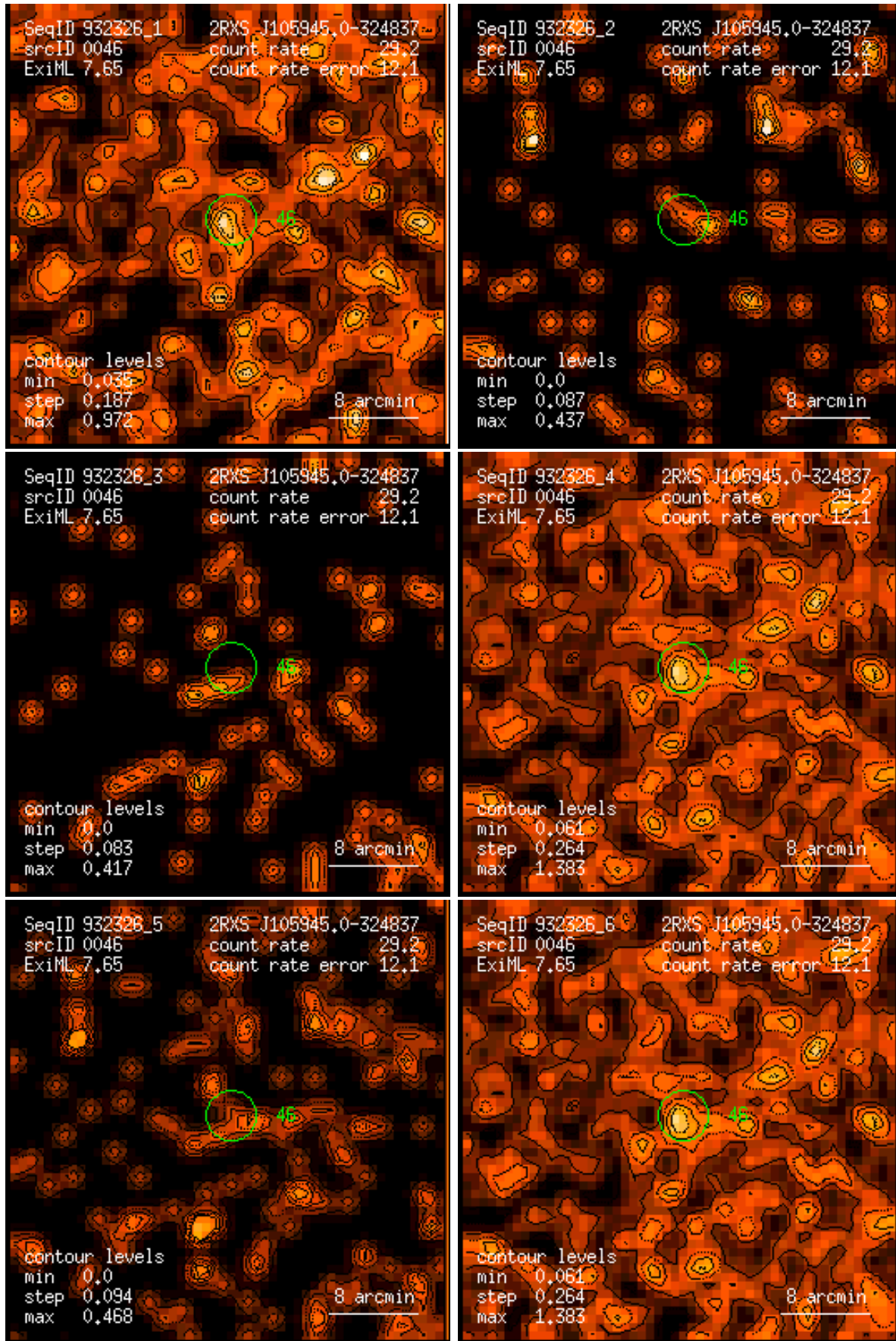
Figure 46: RASS 932326: detection 0046: band rate images, Gaussian filter: (1) PSPC channels 11 – 41, (2) 52 – 90, (3) 91 – 201, (4) 11 – 235, (5) 52 – 201, (6) 11 – 201. Broad band rates in counts/ks. Band rate contour levels in counts/ks/arcmin 2 .
