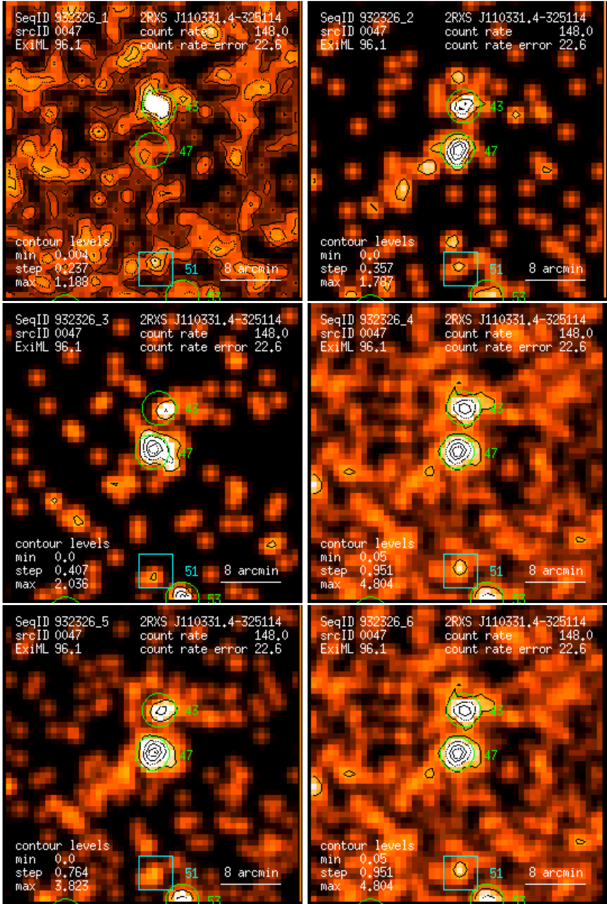
Figure 47: RASS 932326: detection 0047: band rate images, Gaussian filter: (1) PSPC channels 11 – 41, (2) 52 – 90, (3) 91 – 201, (4) 11 – 235, (5) 52 – 201, (6) 11 – 201. Broad band rates in counts/ks. Band rate contour levels in counts/ks/arcmin 2 .
