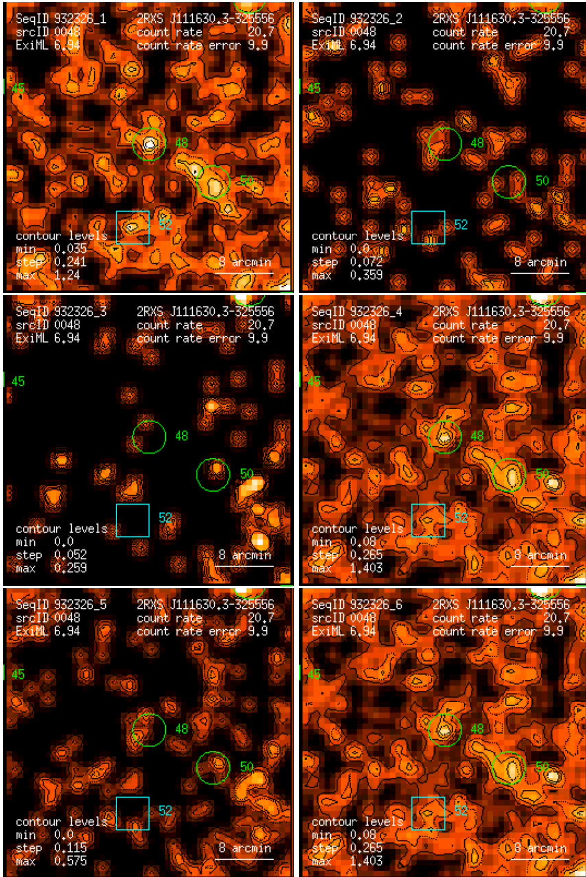
Figure 48: RASS 932326: detection 0048: band rate images, Gaussian filter: (1) PSPC channels 11 – 41, (2) 52 – 90, (3) 91 – 201, (4) 11 – 235, (5) 52 – 201, (6) 11 – 201. Broad band rates in counts/ks. Band rate contour levels in counts/ks/arcmin 2 .
