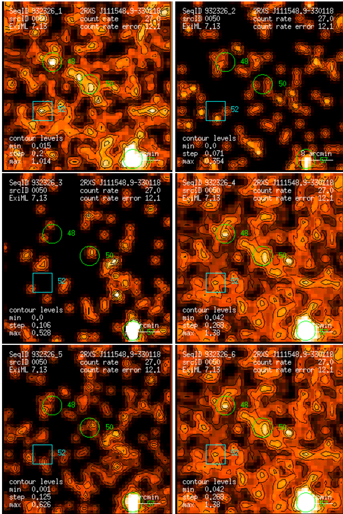
Figure 50: RASS 932326: detection 0050: band rate images, Gaussian filter: (1) PSPC channels 11 – 41, (2) 52 – 90, (3) 91 – 201, (4) 11 – 235, (5) 52 – 201, (6) 11 – 201. Broad band rates in counts/ks. Band rate contour levels in counts/ks/arcmin 2 .
