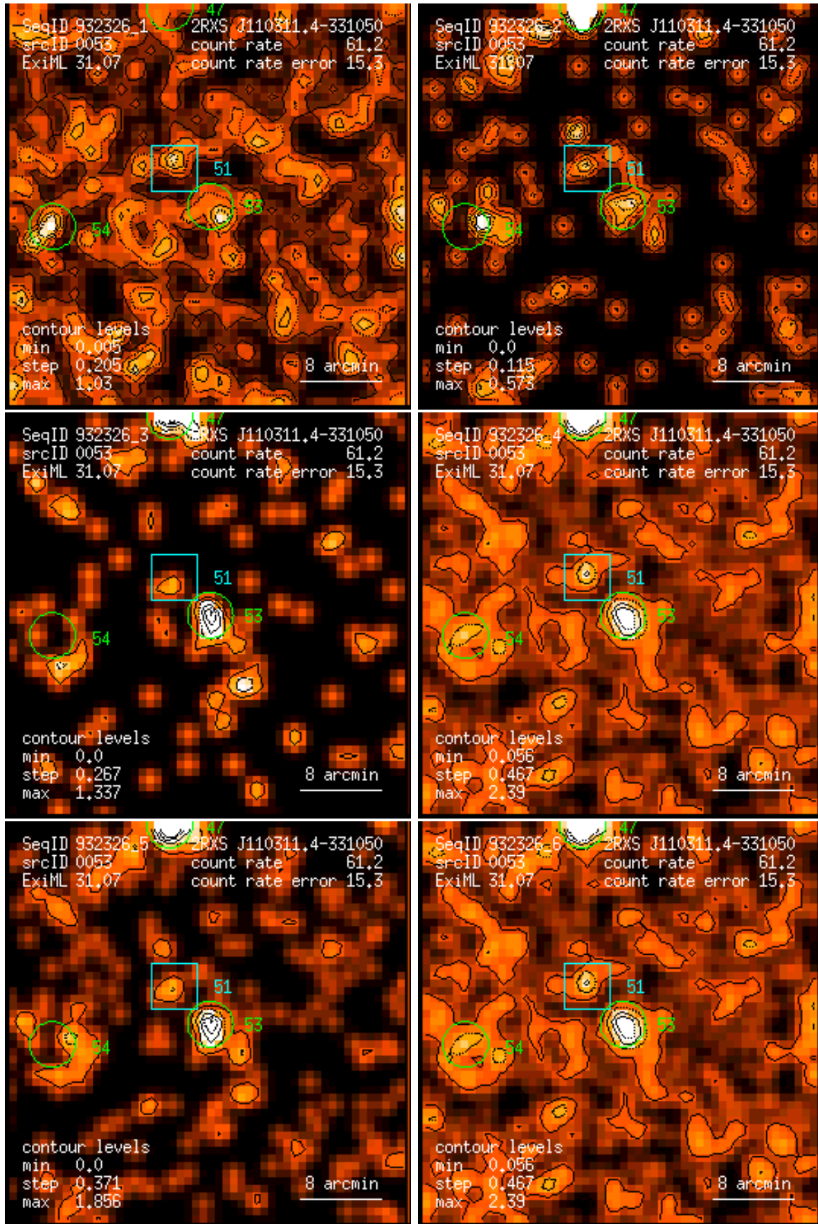
Figure 53: RASS 932326: detection 0053: band rate images, Gaussian filter: (1) PSPC channels 11 – 41, (2) 52 – 90, (3) 91 – 201, (4) 11 – 235, (5) 52 – 201, (6) 11 – 201. Broad band rates in counts/ks. Band rate contour levels in counts/ks/arcmin 2 .
