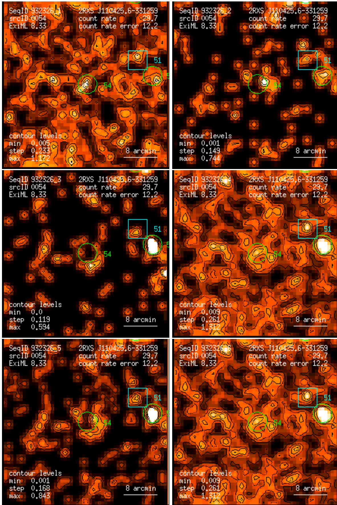
Figure 54: RASS 932326: detection 0054: band rate images, Gaussian filter: (1) PSPC channels 11 – 41, (2) 52 – 90, (3) 91 – 201, (4) 11 – 235, (5) 52 – 201, (6) 11 – 201. Broad band rates in counts/ks. Band rate contour levels in counts/ks/arcmin 2 .
