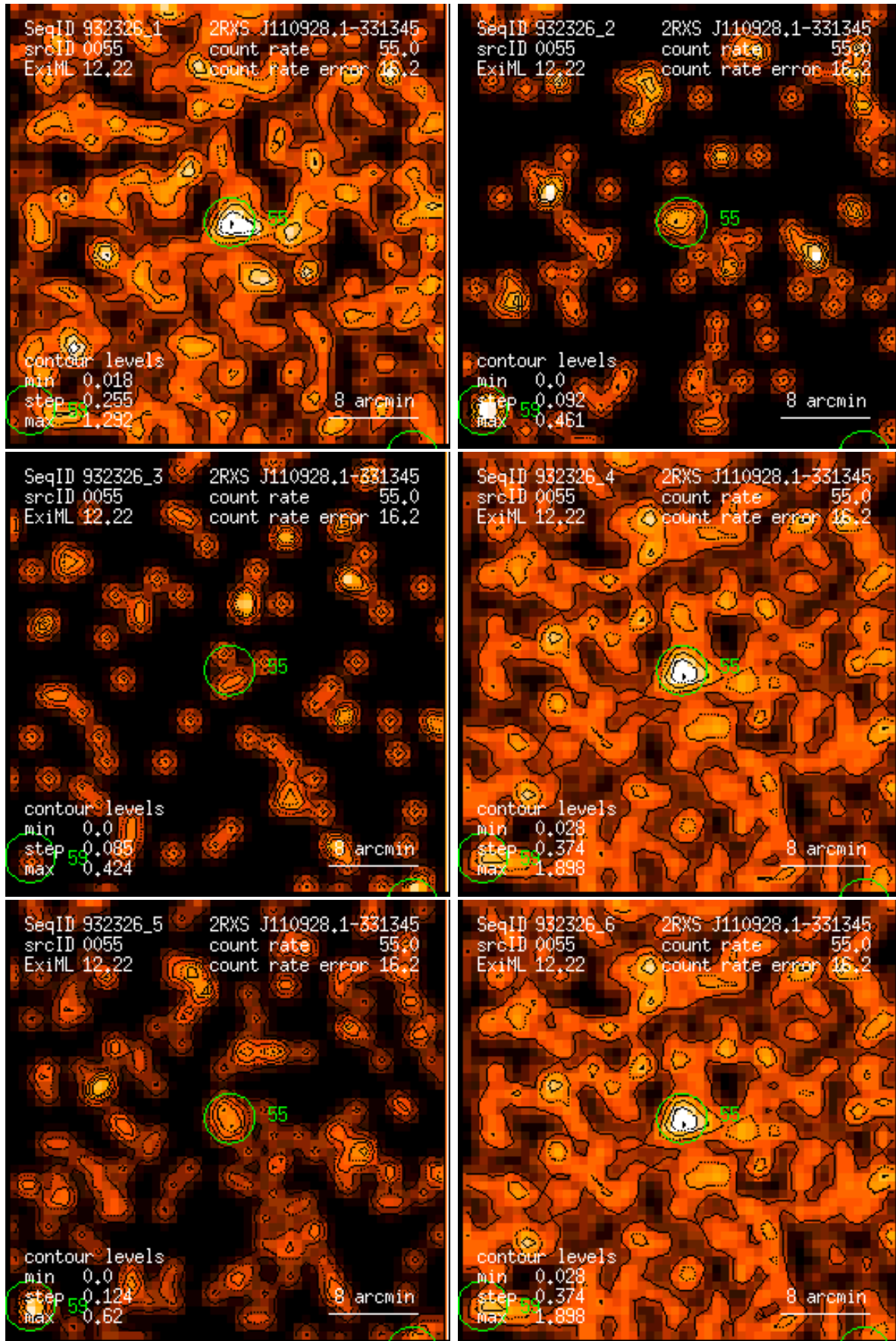
Figure 55: RASS 932326: detection 0055: band rate images, Gaussian filter: (1) PSPC channels 11 – 41, (2) 52 – 90, (3) 91 – 201, (4) 11 – 235, (5) 52 – 201, (6) 11 – 201. Broad band rates in counts/ks. Band rate contour levels in counts/ks/arcmin 2 .
