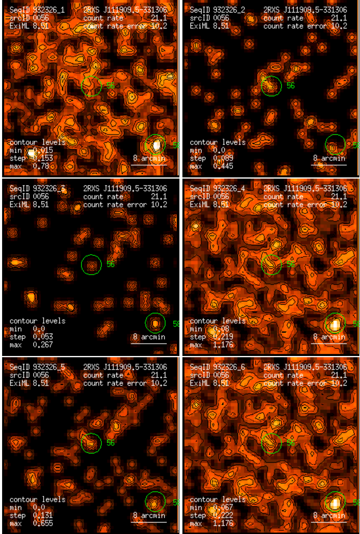
Figure 56: RASS 932326: detection 0056: band rate images, Gaussian filter: (1) PSPC channels 11 – 41, (2) 52 – 90, (3) 91 – 201, (4) 11 – 235, (5) 52 – 201, (6) 11 – 201. Broad band rates in counts/ks. Band rate contour levels in counts/ks/arcmin 2 .
