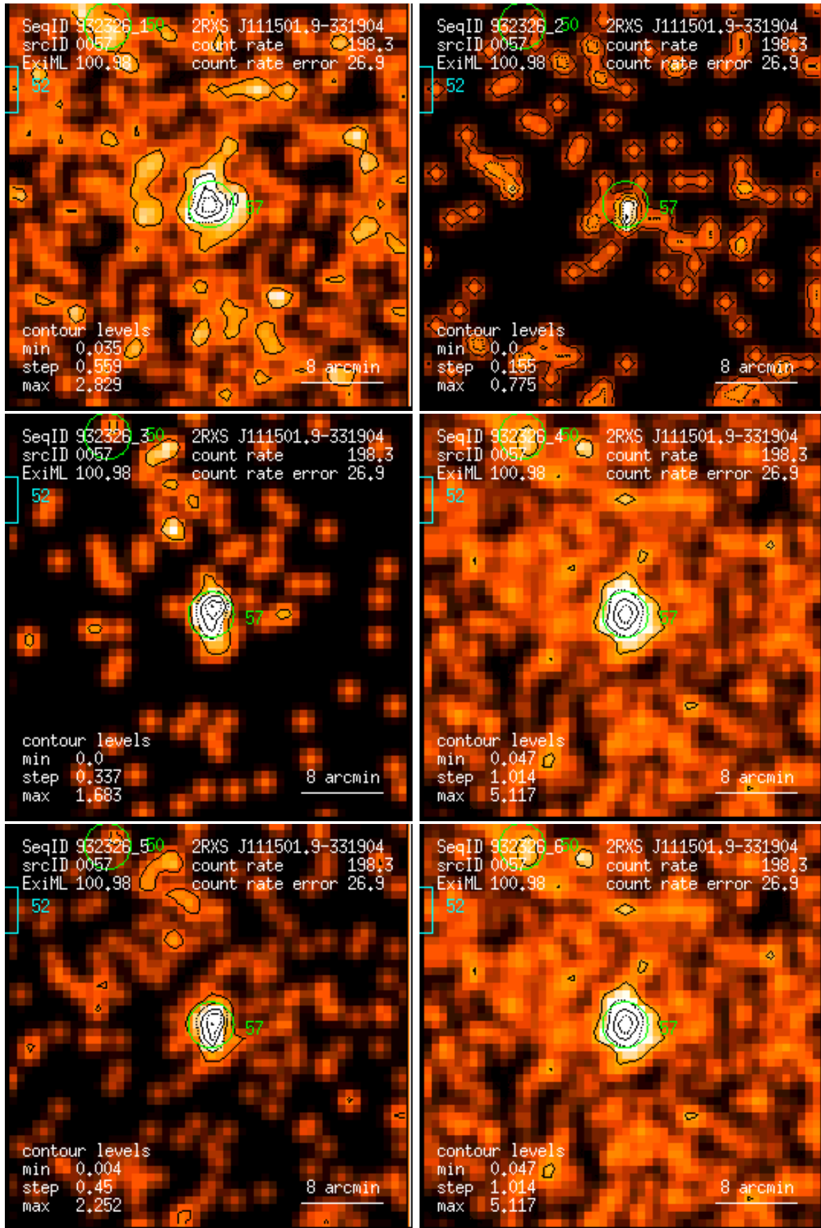
Figure 57: RASS 932326: detection 0057: band rate images, Gaussian filter: (1) PSPC channels 11 – 41, (2) 52 – 90, (3) 91 – 201, (4) 11 – 235, (5) 52 – 201, (6) 11 – 201. Broad band rates in counts/ks. Band rate contour levels in counts/ks/arcmin 2 .
