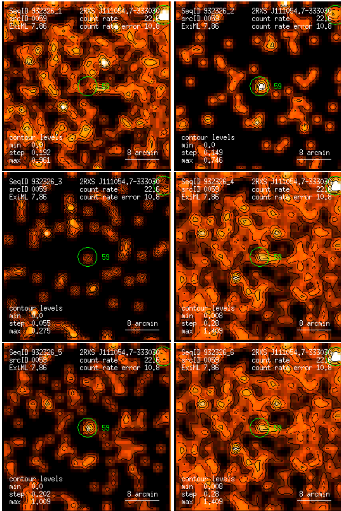
Figure 59: RASS 932326: detection 0059: band rate images, Gaussian filter: (1) PSPC channels 11 – 41, (2) 52 – 90, (3) 91 – 201, (4) 11 – 235, (5) 52 – 201, (6) 11 – 201. Broad band rates in counts/ks. Band rate contour levels in counts/ks/arcmin 2 .
