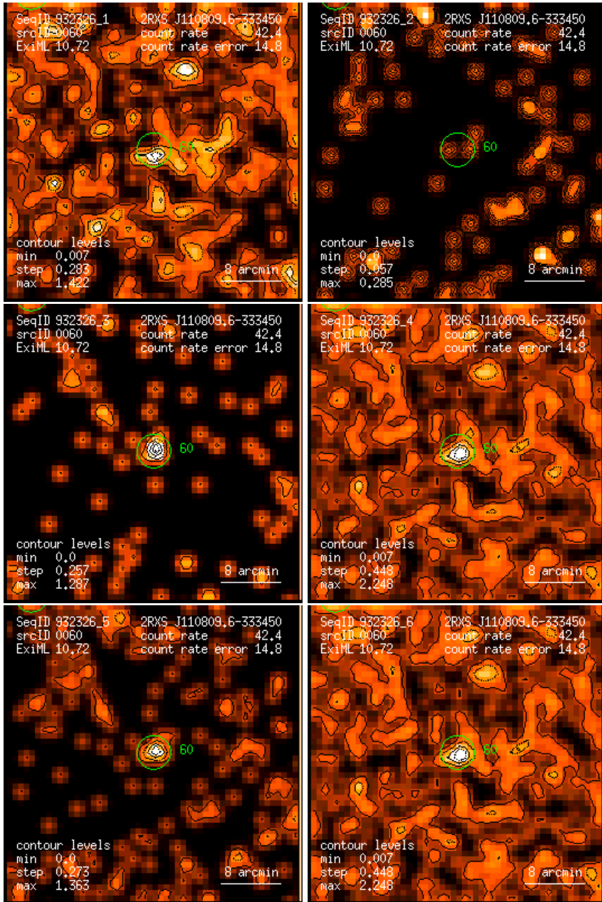
Figure 60: RASS 932326: detection 0060: band rate images, Gaussian filter: (1) PSPC channels 11 – 41, (2) 52 – 90, (3) 91 – 201, (4) 11 – 235, (5) 52 – 201, (6) 11 – 201. Broad band rates in counts/ks. Band rate contour levels in counts/ks/arcmin 2 .
