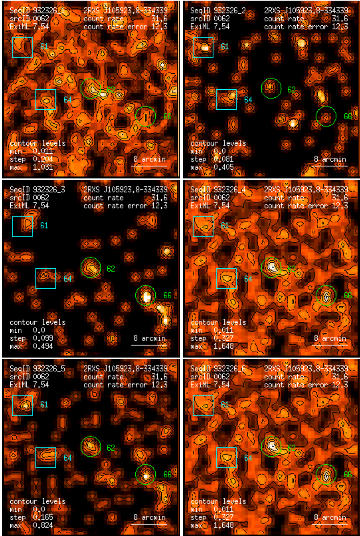
Figure 62: RASS 932326: detection 0062: band rate images, Gaussian filter: (1) PSPC channels 11 – 41, (2) 52 – 90, (3) 91 – 201, (4) 11 – 235, (5) 52 – 201, (6) 11 – 201. Broad band rates in counts/ks. Band rate contour levels in counts/ks/arcmin 2 .
