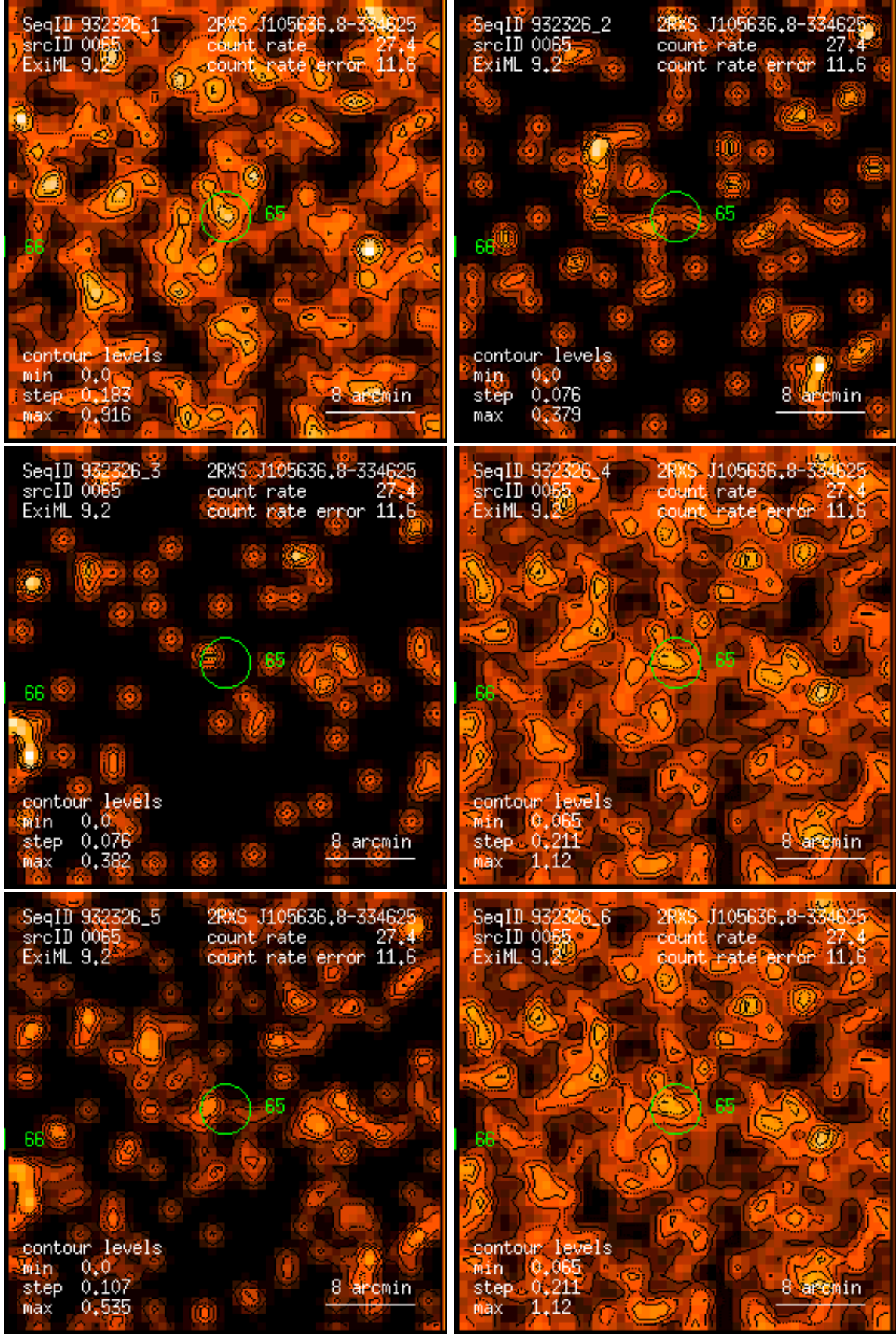
Figure 65: RASS 932326: detection 0065: band rate images, Gaussian filter: (1) PSPC channels 11 – 41, (2) 52 – 90, (3) 91 – 201, (4) 11 – 235, (5) 52 – 201, (6) 11 – 201. Broad band rates in counts/ks. Band rate contour levels in counts/ks/arcmin 2 .
