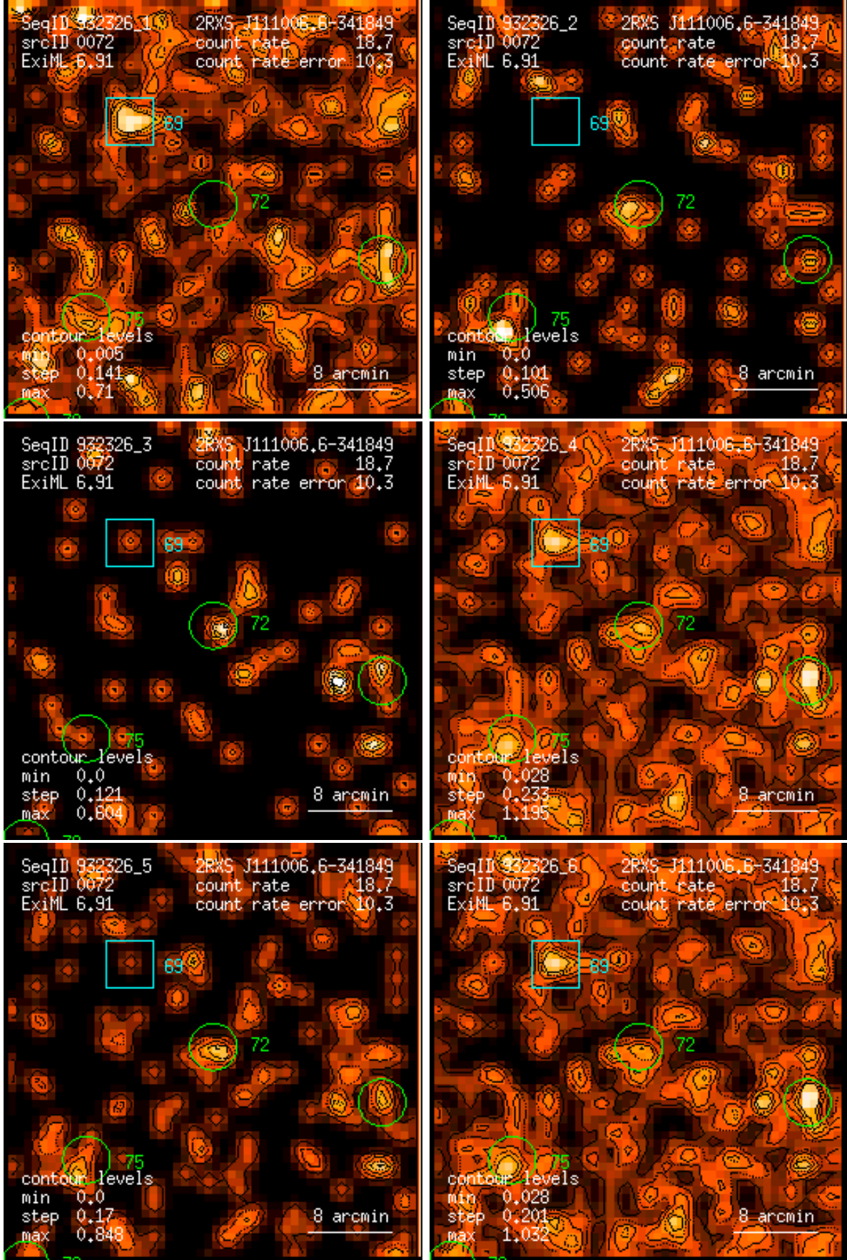
Figure 72: RASS 932326: detection 0072: band rate images, Gaussian filter: (1) PSPC channels 11 – 41, (2) 52 – 90, (3) 91 – 201, (4) 11 – 235, (5) 52 – 201, (6) 11 – 201. Broad band rates in counts/ks. Band rate contour levels in counts/ks/arcmin 2 .
