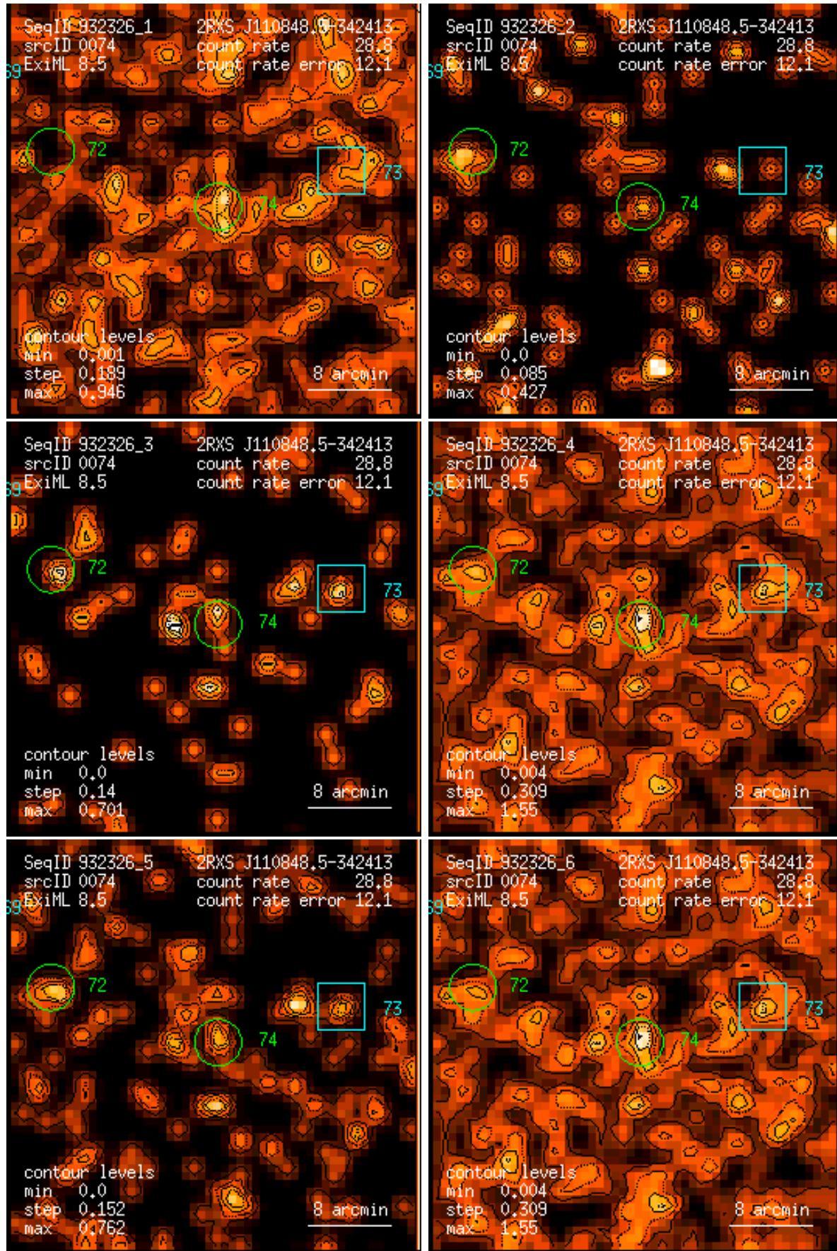
Figure 74: RASS 932326: detection 0074: band rate images, Gaussian filter: (1) PSPC channels 11 – 41, (2) 52 – 90, (3) 91 – 201, (4) 11 – 235, (5) 52 – 201, (6) 11 – 201. Broad band rates in counts/ks. Band rate contour levels in counts/ks/arcmin 2 .
