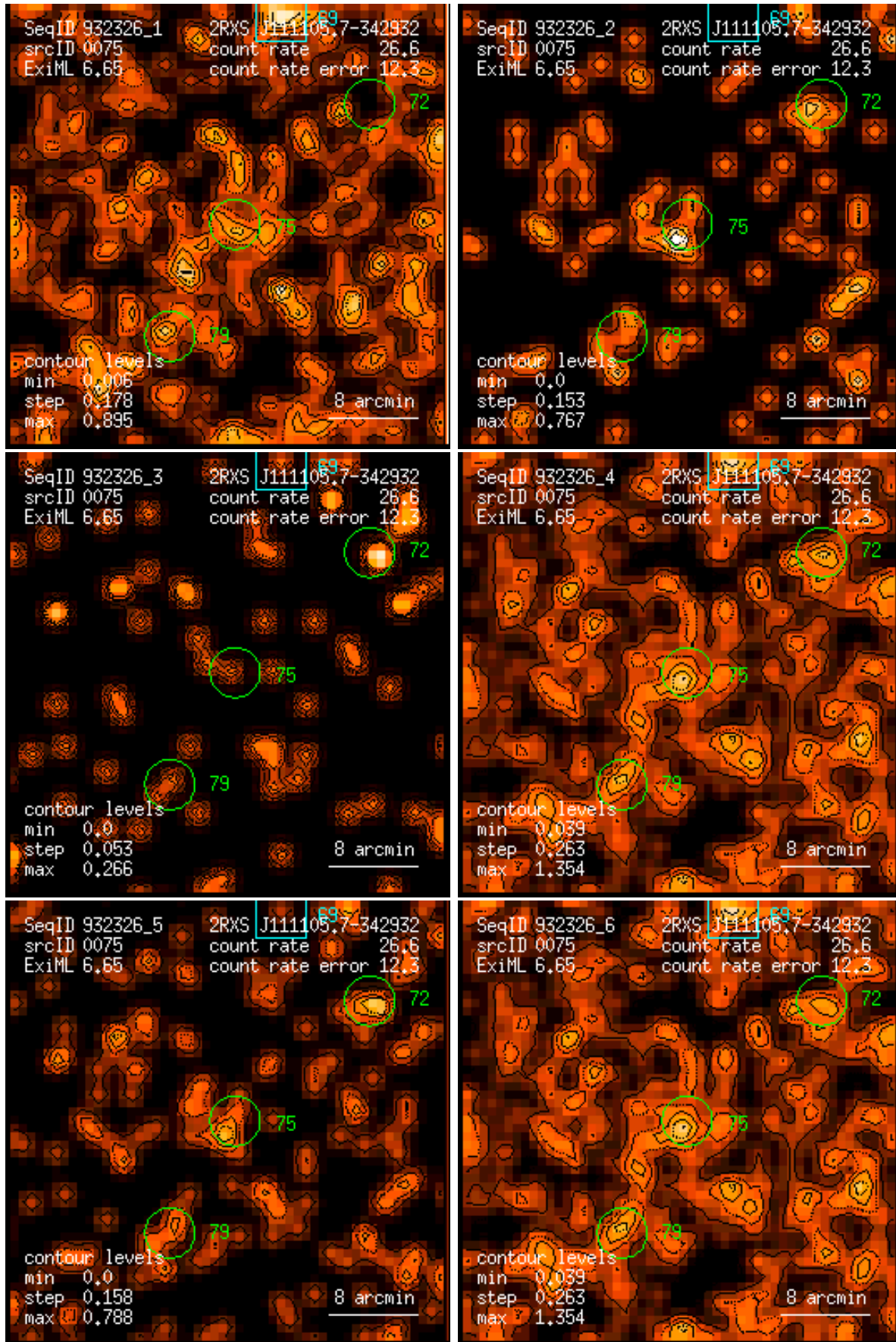
Figure 75: RASS 932326: detection 0075: band rate images, Gaussian filter: (1) PSPC channels 11 – 41, (2) 52 – 90, (3) 91 – 201, (4) 11 – 235, (5) 52 – 201, (6) 11 – 201. Broad band rates in counts/ks. Band rate contour levels in counts/ks/arcmin 2 .
