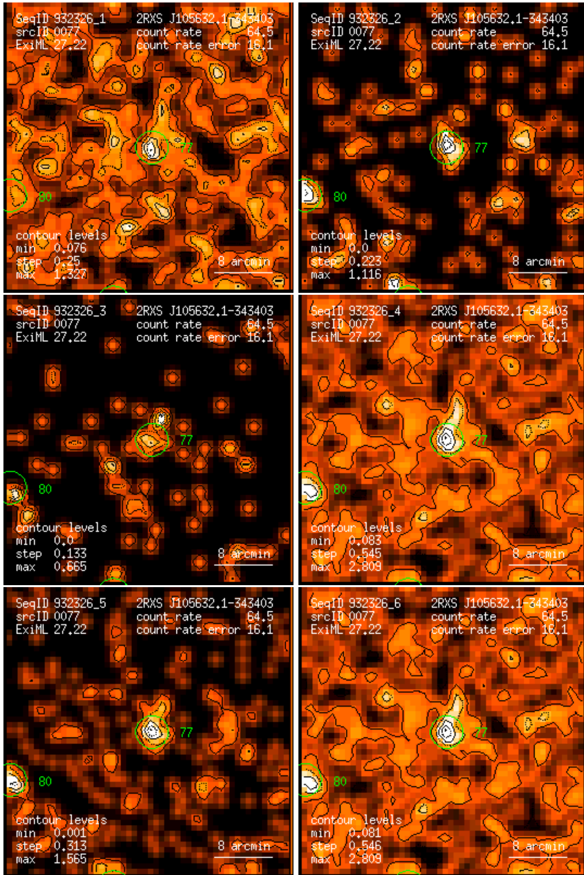
Figure 77: RASS 932326: detection 0077: band rate images, Gaussian filter: (1) PSPC channels 11 – 41, (2) 52 – 90, (3) 91 – 201, (4) 11 – 235, (5) 52 – 201, (6) 11 – 201. Broad band rates in counts/ks. Band rate contour levels in counts/ks/arcmin 2 .
