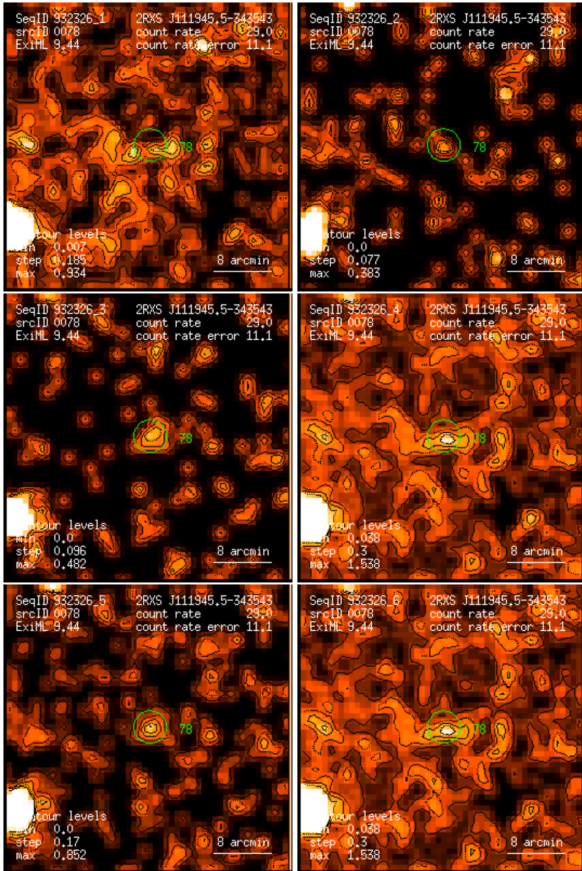
Figure 78: RASS 932326: detection 0078: band rate images, Gaussian filter: (1) PSPC channels 11 – 41, (2) 52 – 90, (3) 91 – 201, (4) 11 – 235, (5) 52 – 201, (6) 11 – 201. Broad band rates in counts/ks. Band rate contour levels in counts/ks/arcmin 2 .
