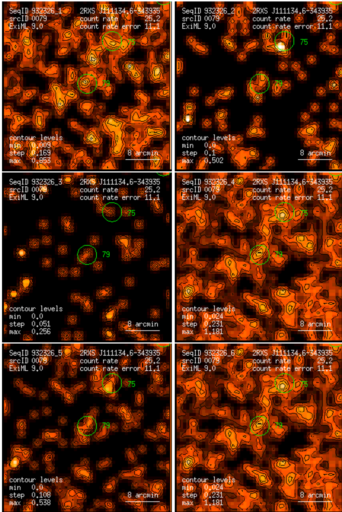
Figure 79: RASS 932326: detection 0079: band rate images, Gaussian filter: (1) PSPC channels 11 – 41, (2) 52 – 90, (3) 91 – 201, (4) 11 – 235, (5) 52 – 201, (6) 11 – 201. Broad band rates in counts/ks. Band rate contour levels in counts/ks/arcmin 2 .
