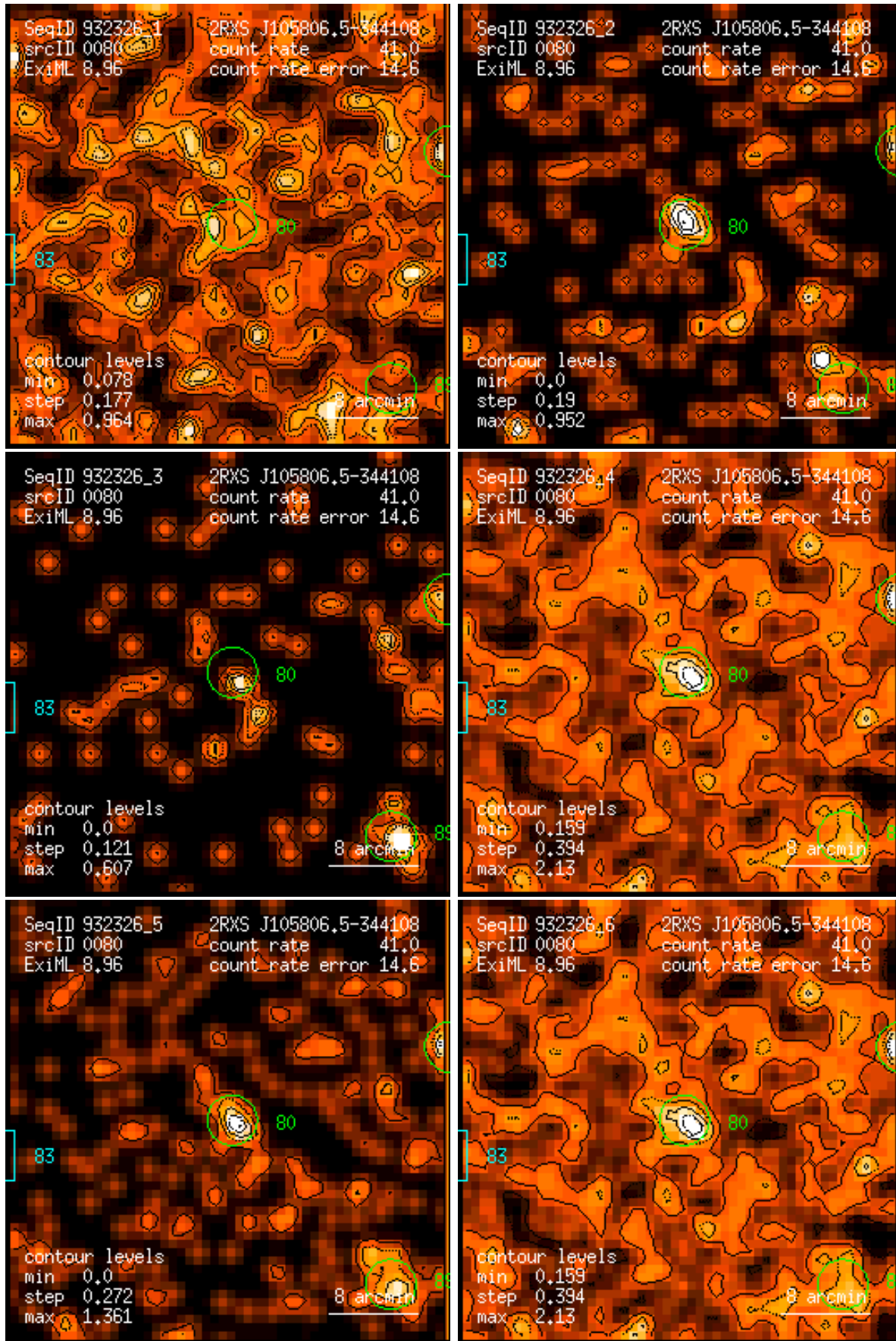
Figure 80: RASS 932326: detection 0080: band rate images, Gaussian filter: (1) PSPC channels 11 – 41, (2) 52 – 90, (3) 91 – 201, (4) 11 – 235, (5) 52 – 201, (6) 11 – 201. Broad band rates in counts/ks. Band rate contour levels in counts/ks/arcmin 2 .
