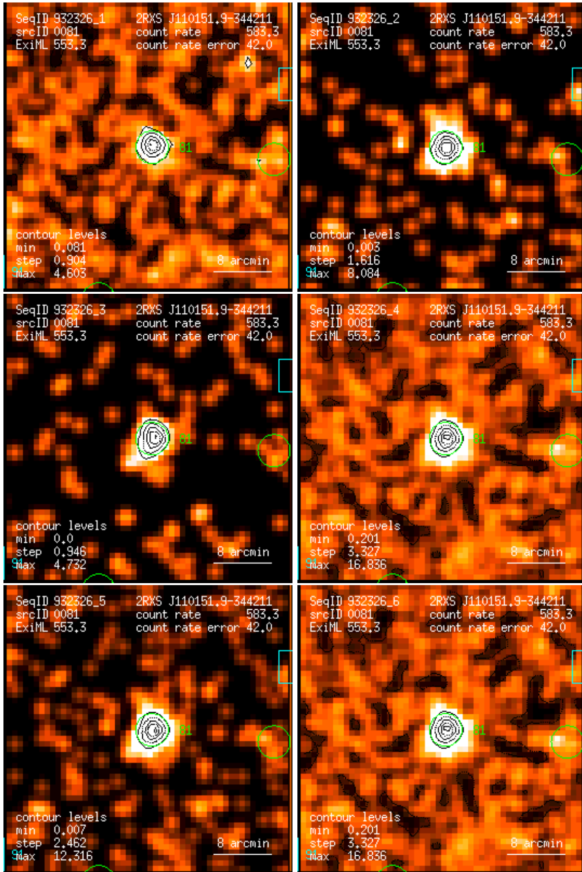
Figure 81: RASS 932326: detection 0081: band rate images, Gaussian filter: (1) PSPC channels 11 – 41, (2) 52 – 90, (3) 91 – 201, (4) 11 – 235, (5) 52 – 201, (6) 11 – 201. Broad band rates in counts/ks. Band rate contour levels in counts/ks/arcmin 2 .
