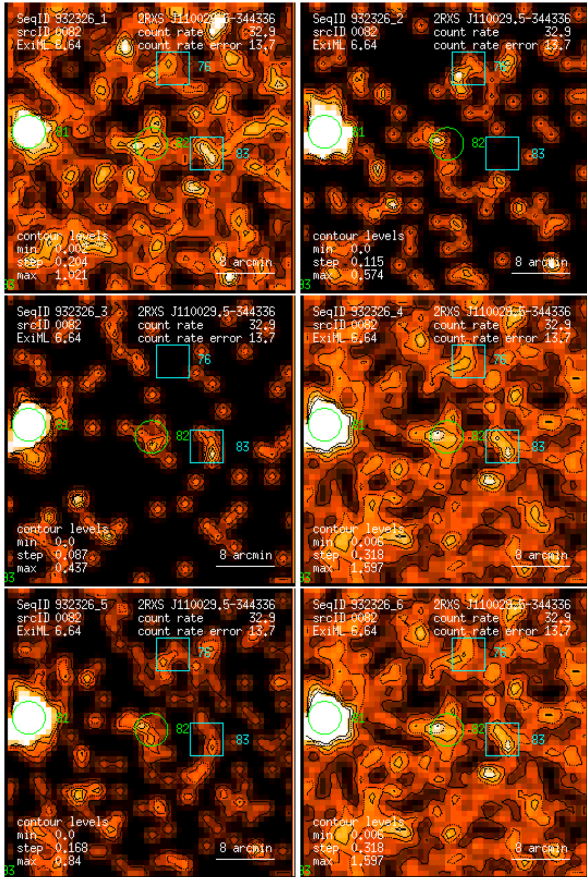
Figure 82: RASS 932326: detection 0082: band rate images, Gaussian filter: (1) PSPC channels 11 – 41, (2) 52 – 90, (3) 91 – 201, (4) 11 – 235, (5) 52 – 201, (6) 11 – 201. Broad band rates in counts/ks. Band rate contour levels in counts/ks/arcmin 2 .
