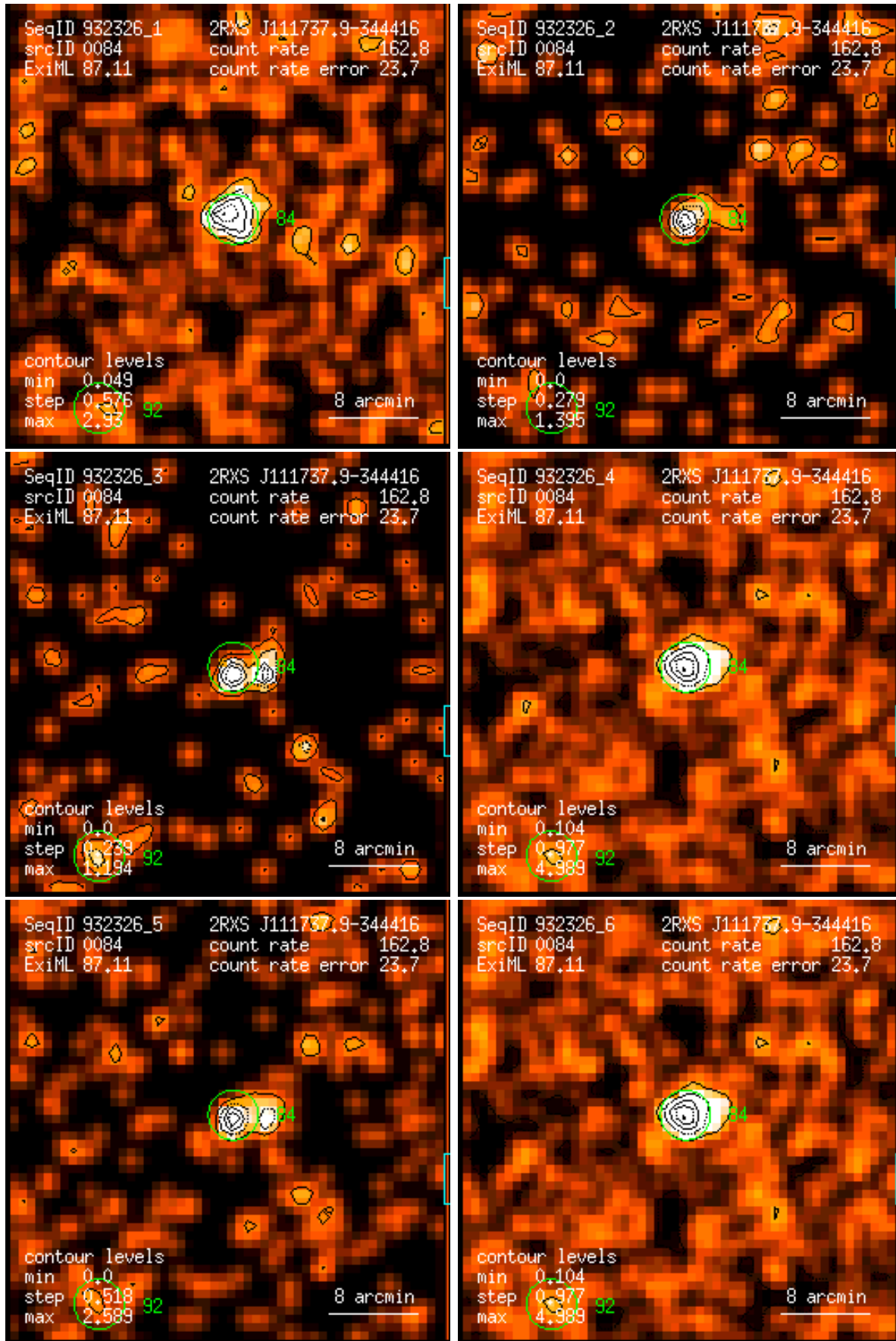
Figure 84: RASS 932326: detection 0084: band rate images, Gaussian filter: (1) PSPC channels 11 – 41, (2) 52 – 90, (3) 91 – 201, (4) 11 – 235, (5) 52 – 201, (6) 11 – 201. Broad band rates in counts/ks. Band rate contour levels in counts/ks/arcmin 2 .
