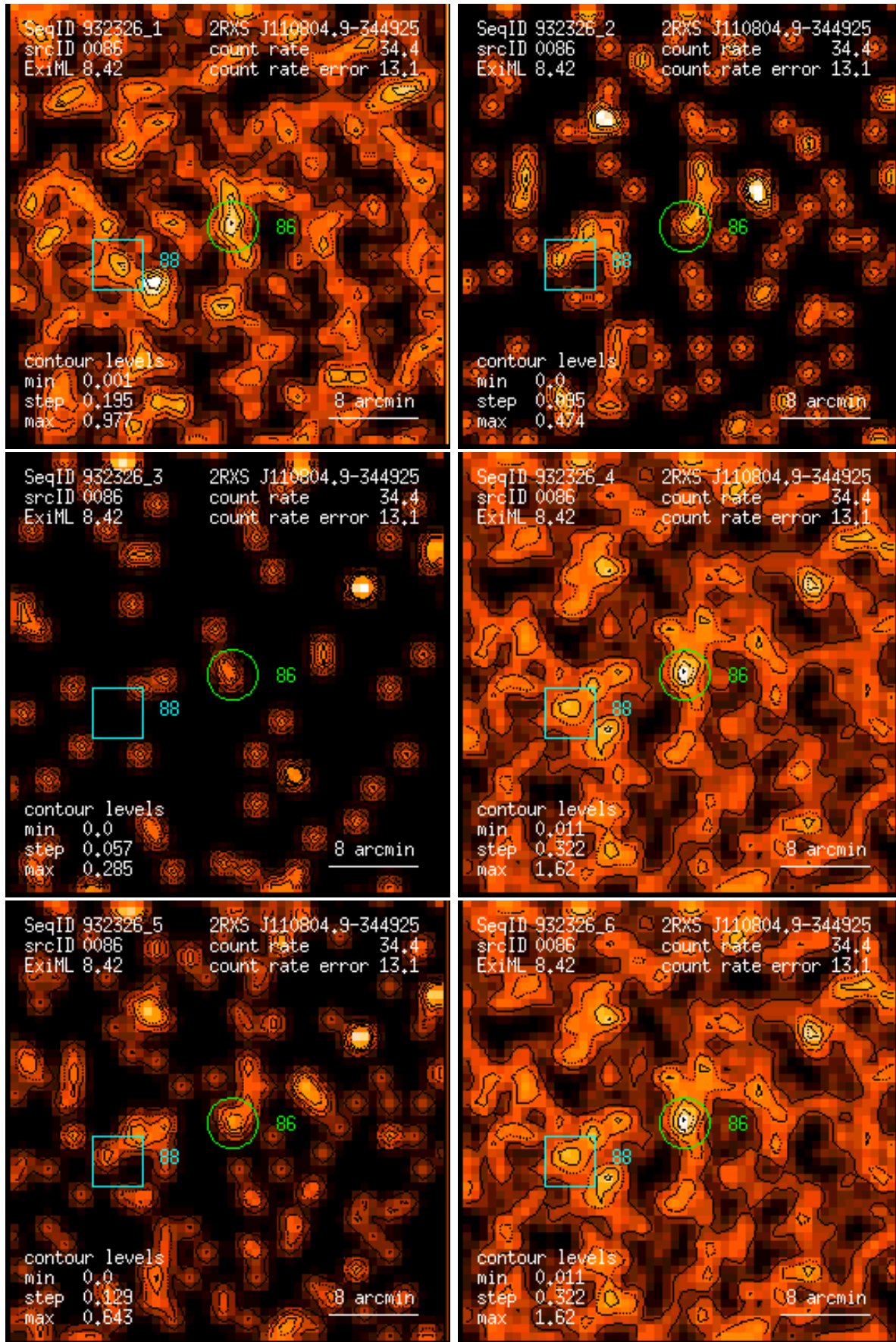
Figure 86: RASS 932326: detection 0086: band rate images, Gaussian filter: (1) PSPC channels 11 – 41, (2) 52 – 90, (3) 91 – 201, (4) 11 – 235, (5) 52 – 201, (6) 11 – 201. Broad band rates in counts/ks. Band rate contour levels in counts/ks/arcmin 2 .
