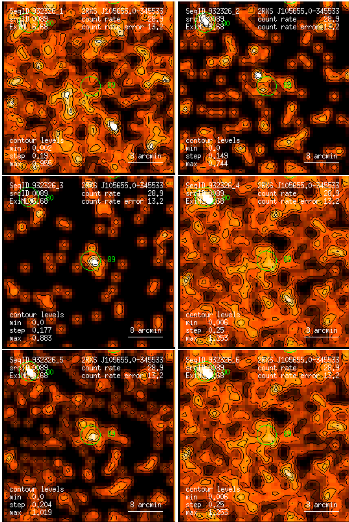
Figure 89: RASS 932326: detection 0089: band rate images, Gaussian filter: (1) PSPC channels 11 – 41, (2) 52 – 90, (3) 91 – 201, (4) 11 – 235, (5) 52 – 201, (6) 11 – 201. Broad band rates in counts/ks. Band rate contour levels in counts/ks/arcmin 2 .
