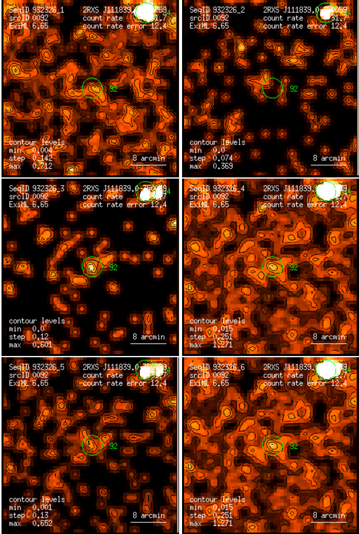
Figure 92: RASS 932326: detection 0092: band rate images, Gaussian filter: (1) PSPC channels 11 – 41, (2) 52 – 90, (3) 91 – 201, (4) 11 – 235, (5) 52 – 201, (6) 11 – 201. Broad band rates in counts/ks. Band rate contour levels in counts/ks/arcmin 2 .
