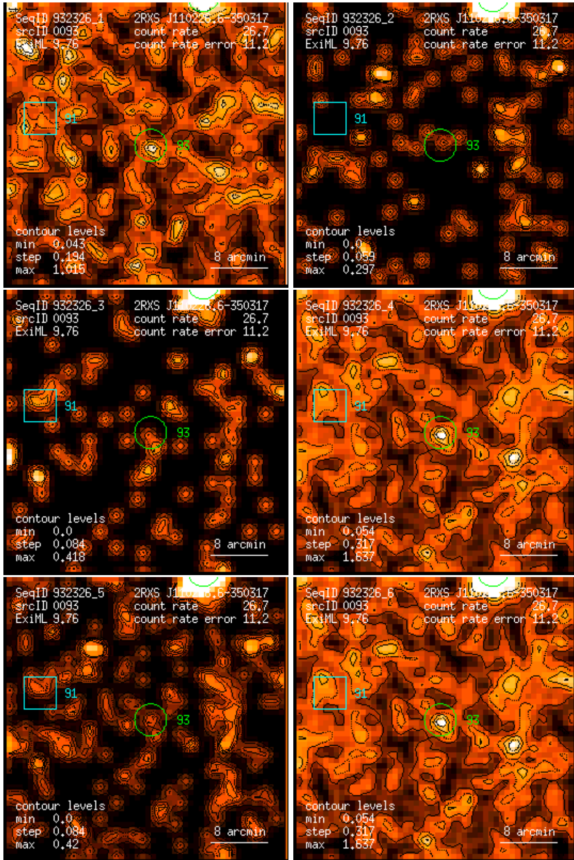
Figure 93: RASS 932326: detection 0093: band rate images, Gaussian filter: (1) PSPC channels 11 – 41, (2) 52 – 90, (3) 91 – 201, (4) 11 – 235, (5) 52 – 201, (6) 11 – 201. Broad band rates in counts/ks. Band rate contour levels in counts/ks/arcmin 2 .
