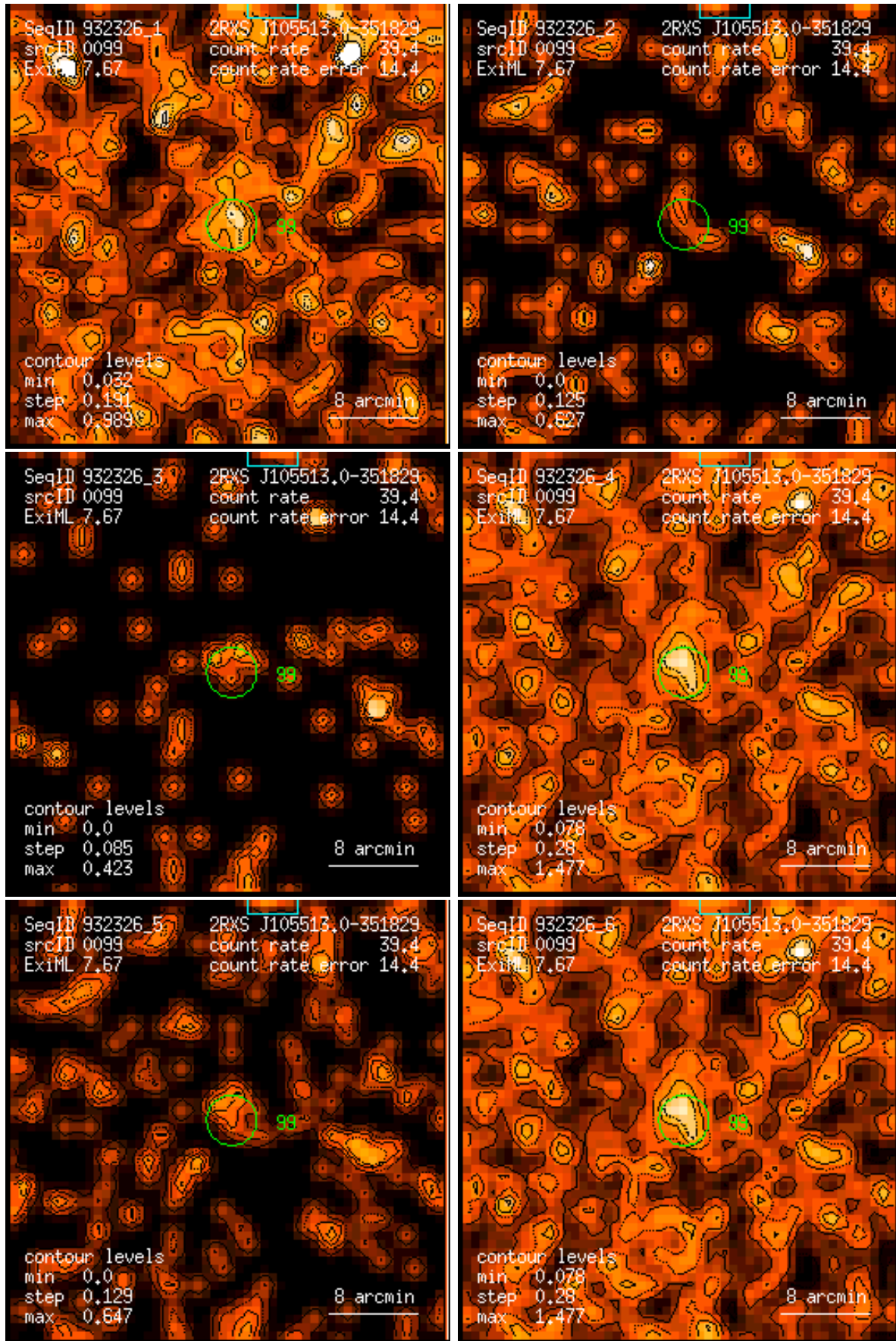
Figure 99: RASS 932326: detection 0099: band rate images, Gaussian filter: (1) PSPC channels 11 – 41, (2) 52 – 90, (3) 91 – 201, (4) 11 – 235, (5) 52 – 201, (6) 11 – 201. Broad band rates in counts/ks. Band rate contour levels in counts/ks/arcmin 2 .
