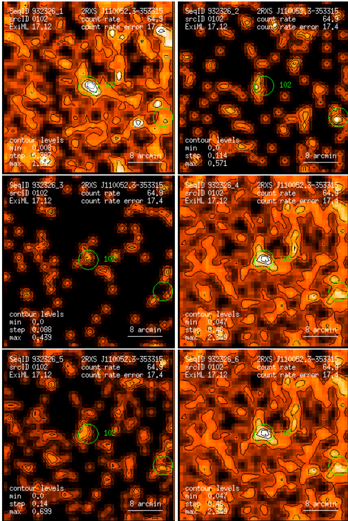
Figure 102: RASS 932326: detection 0102: band rate images, Gaussian filter: (1) PSPC channels 11 – 41, (2) 52 – 90, (3) 91 – 201, (4) 11 – 235, (5) 52 – 201, (6) 11 – 201. Broad band rates in counts/ks. Band rate contour levels in counts/ks/arcmin 2 .
