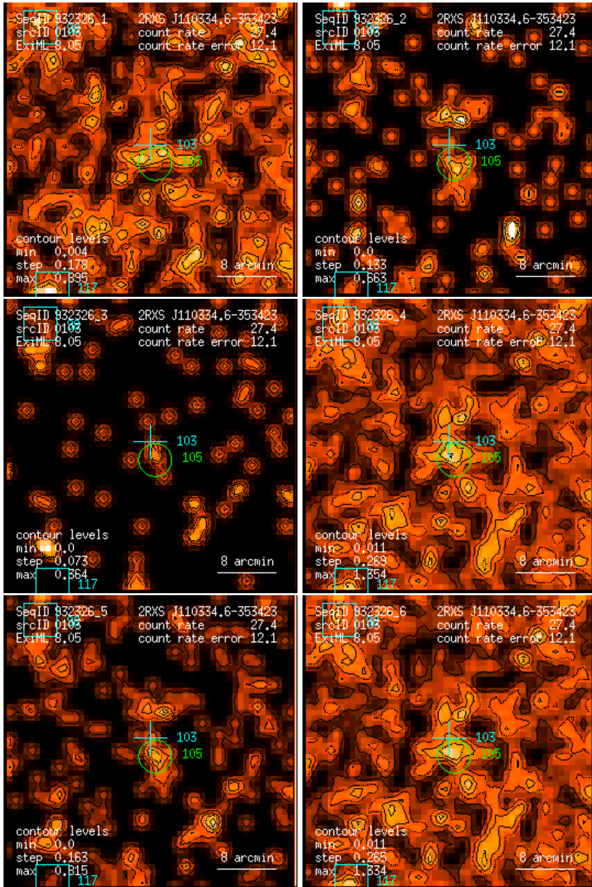
Figure 103: RASS 932326: detection 0103: band rate images, Gaussian filter: (1) PSPC channels 11 – 41, (2) 52 – 90, (3) 91 – 201, (4) 11 – 235, (5) 52 – 201, (6) 11 – 201. Broad band rates in counts/ks. Band rate contour levels in counts/ks/arcmin 2 .
