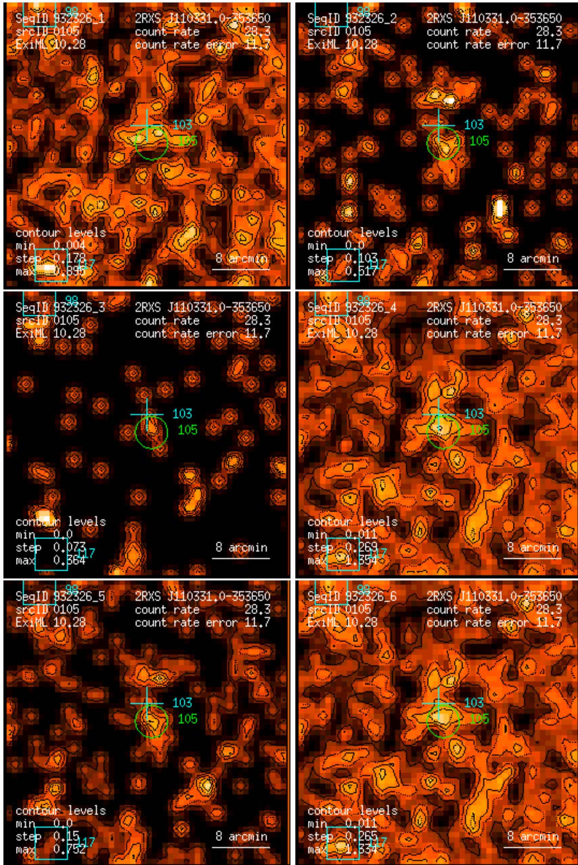
Figure 105: RASS 932326: detection 0105: band rate images, Gaussian filter: (1) PSPC channels 11 – 41, (2) 52 – 90, (3) 91 – 201, (4) 11 – 235, (5) 52 – 201, (6) 11 – 201. Broad band rates in counts/ks. Band rate contour levels in counts/ks/arcmin 2 .
