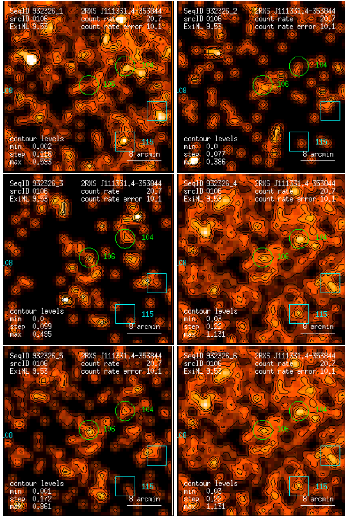
Figure 106: RASS 932326: detection 0106: band rate images, Gaussian filter: (1) PSPC channels 11 – 41, (2) 52 – 90, (3) 91 – 201, (4) 11 – 235, (5) 52 – 201, (6) 11 – 201. Broad band rates in counts/ks. Band rate contour levels in counts/ks/arcmin 2 .
