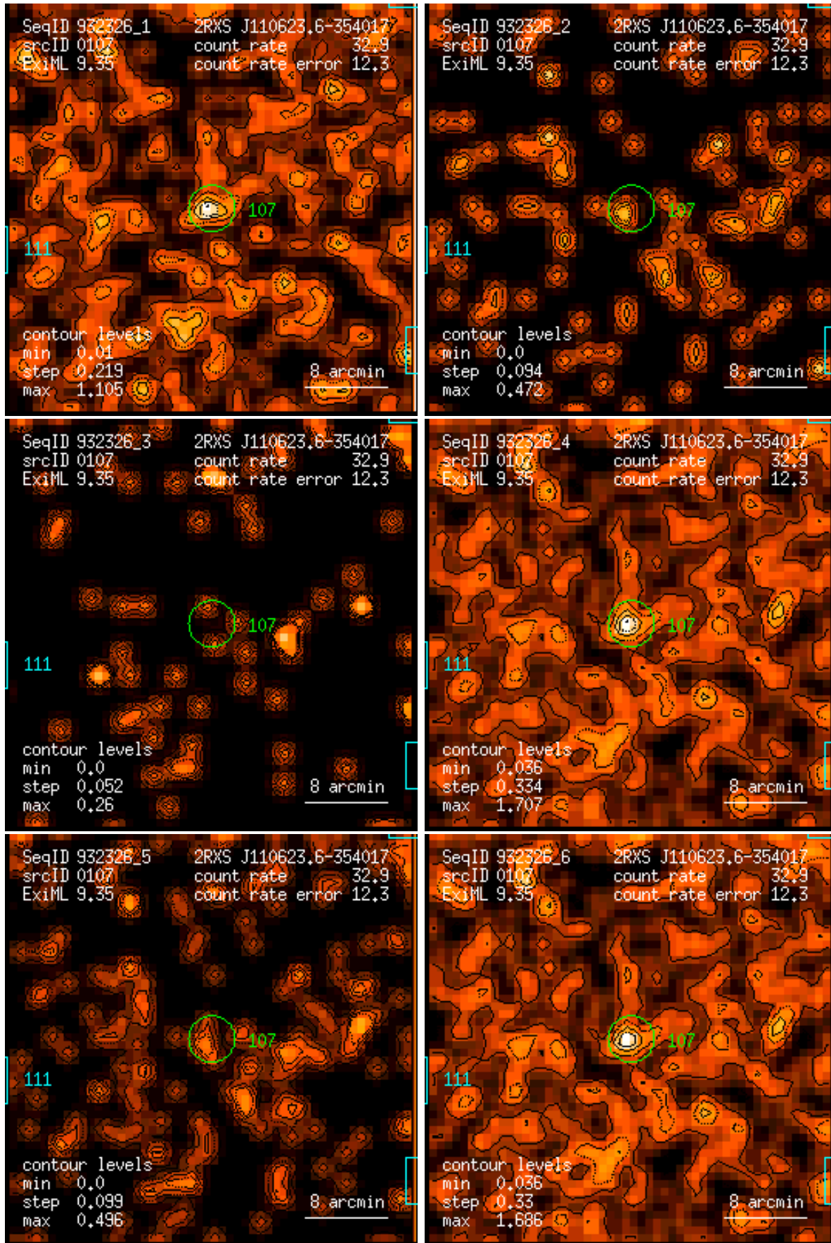
Figure 107: RASS 932326: detection 0107: band rate images, Gaussian filter: (1) PSPC channels 11 – 41, (2) 52 – 90, (3) 91 – 201, (4) 11 – 235, (5) 52 – 201, (6) 11 – 201. Broad band rates in counts/ks. Band rate contour levels in counts/ks/arcmin 2 .
