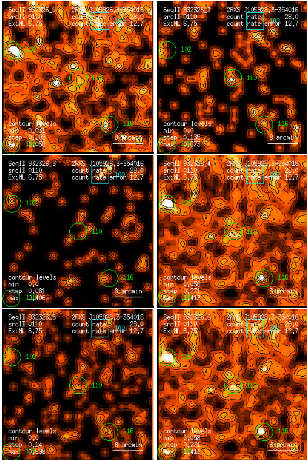
Figure 110: RASS 932326: detection 0110: band rate images, Gaussian filter: (1) PSPC channels 11 – 41, (2) 52 – 90, (3) 91 – 201, (4) 11 – 235, (5) 52 – 201, (6) 11 – 201. Broad band rates in counts/ks. Band rate contour levels in counts/ks/arcmin 2 .
