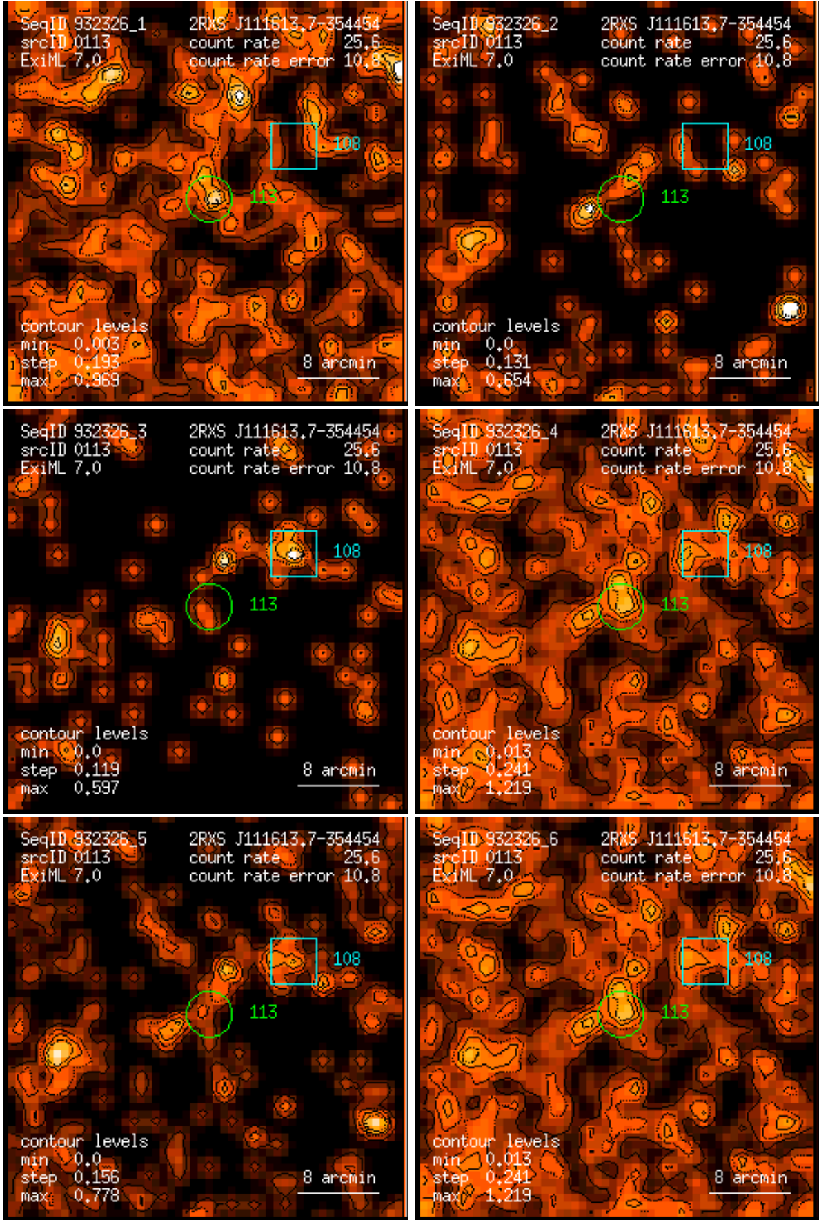
Figure 113: RASS 932326: detection 0113: band rate images, Gaussian filter: (1) PSPC channels 11 – 41, (2) 52 – 90, (3) 91 – 201, (4) 11 – 235, (5) 52 – 201, (6) 11 – 201. Broad band rates in counts/ks. Band rate contour levels in counts/ks/arcmin 2 .
