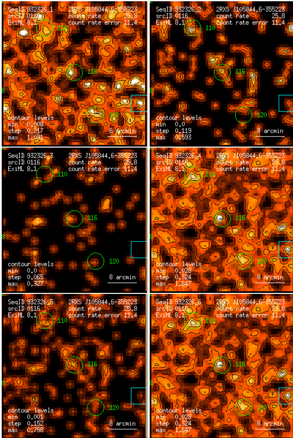
Figure 116: RASS 932326: detection 0116: band rate images, Gaussian filter: (1) PSPC channels 11 – 41, (2) 52 – 90, (3) 91 – 201, (4) 11 – 235, (5) 52 – 201, (6) 11 – 201. Broad band rates in counts/ks. Band rate contour levels in counts/ks/arcmin 2 .
