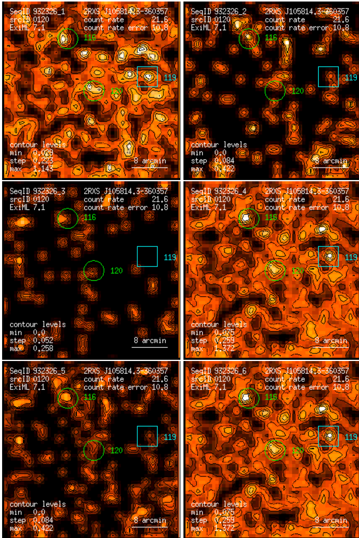
Figure 120: RASS 932326: detection 0120: band rate images, Gaussian filter: (1) PSPC channels 11 – 41, (2) 52 – 90, (3) 91 – 201, (4) 11 – 235, (5) 52 – 201, (6) 11 – 201. Broad band rates in counts/ks. Band rate contour levels in counts/ks/arcmin 2 .
