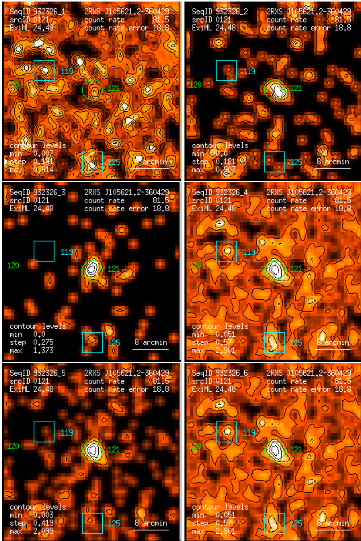
Figure 121: RASS 932326: detection 0121: band rate images, Gaussian filter: (1) PSPC channels 11 – 41, (2) 52 – 90, (3) 91 – 201, (4) 11 – 235, (5) 52 – 201, (6) 11 – 201. Broad band rates in counts/ks. Band rate contour levels in counts/ks/arcmin 2 .
