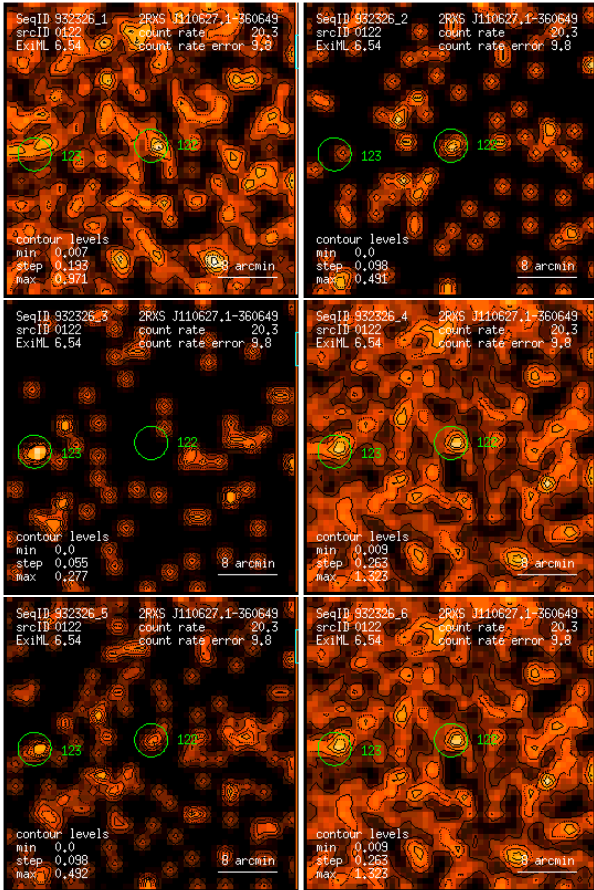
Figure 122: RASS 932326: detection 0122: band rate images, Gaussian filter: (1) PSPC channels 11 – 41, (2) 52 – 90, (3) 91 – 201, (4) 11 – 235, (5) 52 – 201, (6) 11 – 201. Broad band rates in counts/ks. Band rate contour levels in counts/ks/arcmin 2 .
