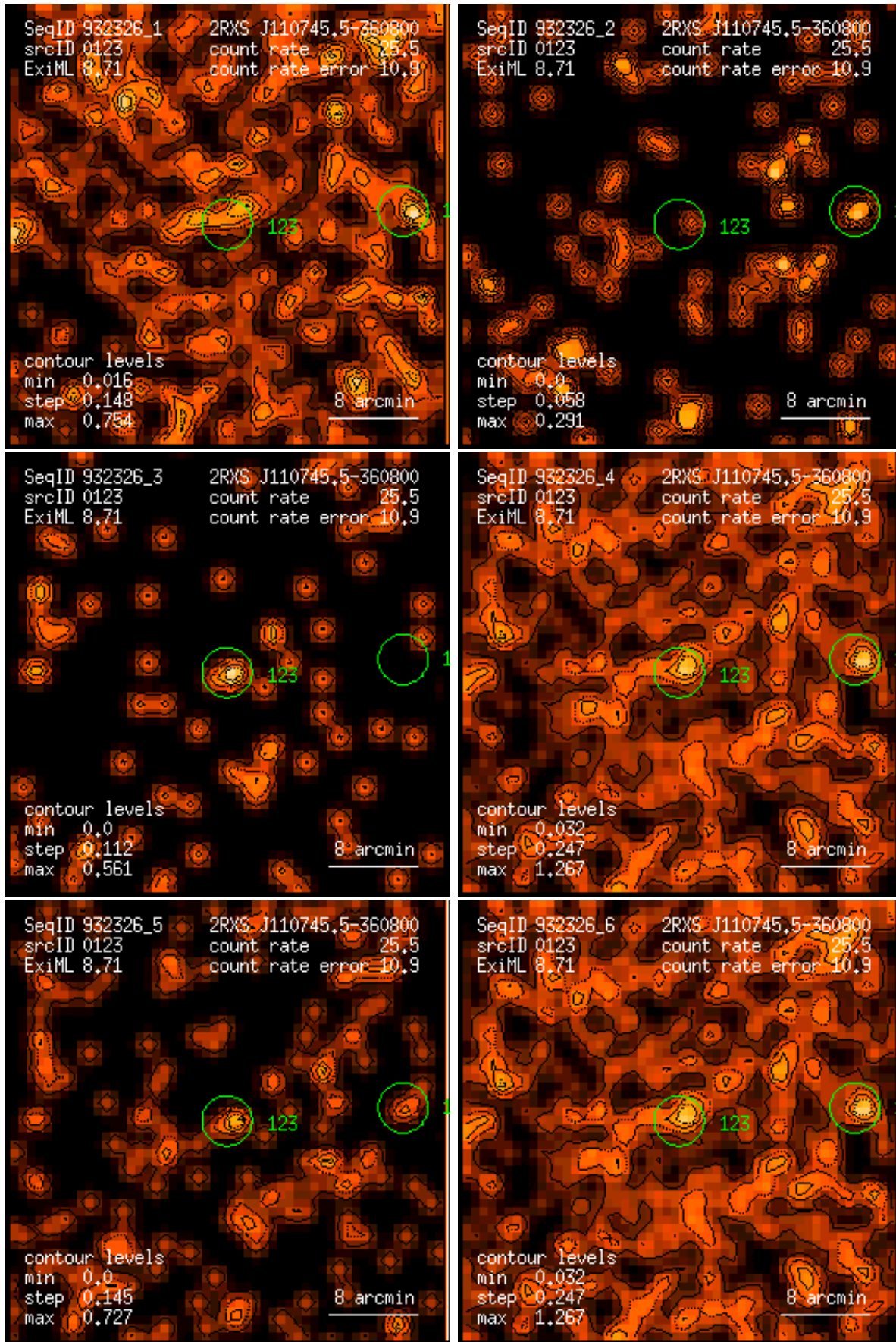
Figure 123: RASS 932326: detection 0123: band rate images, Gaussian filter: (1) PSPC channels 11 – 41, (2) 52 – 90, (3) 91 – 201, (4) 11 – 235, (5) 52 – 201, (6) 11 – 201. Broad band rates in counts/ks. Band rate contour levels in counts/ks/arcmin 2 .
