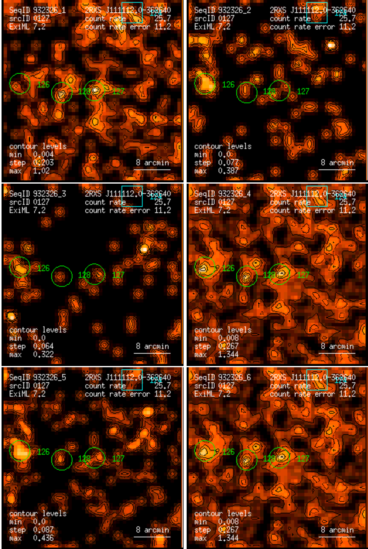
Figure 127: RASS 932326: detection 0127: band rate images, Gaussian filter: (1) PSPC channels 11 – 41, (2) 52 – 90, (3) 91 – 201, (4) 11 – 235, (5) 52 – 201, (6) 11 – 201. Broad band rates in counts/ks. Band rate contour levels in counts/ks/arcmin 2 .
