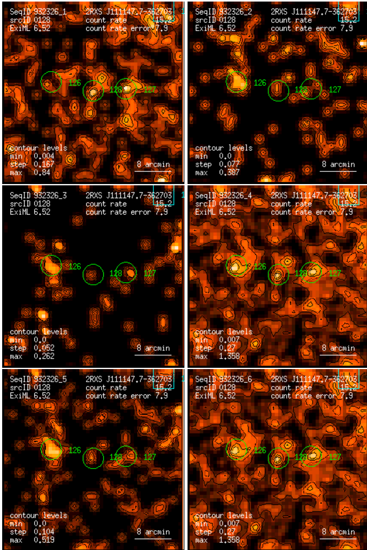
Figure 128: RASS 932326: detection 0128: band rate images, Gaussian filter: (1) PSPC channels 11 – 41, (2) 52 – 90, (3) 91 – 201, (4) 11 – 235, (5) 52 – 201, (6) 11 – 201. Broad band rates in counts/ks. Band rate contour levels in counts/ks/arcmin 2 .
