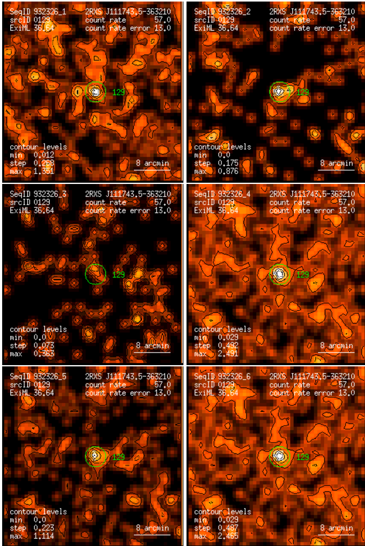
Figure 129: RASS 932326: detection 0129: band rate images, Gaussian filter: (1) PSPC channels 11 – 41, (2) 52 – 90, (3) 91 – 201, (4) 11 – 235, (5) 52 – 201, (6) 11 – 201. Broad band rates in counts/ks. Band rate contour levels in counts/ks/arcmin 2 .
