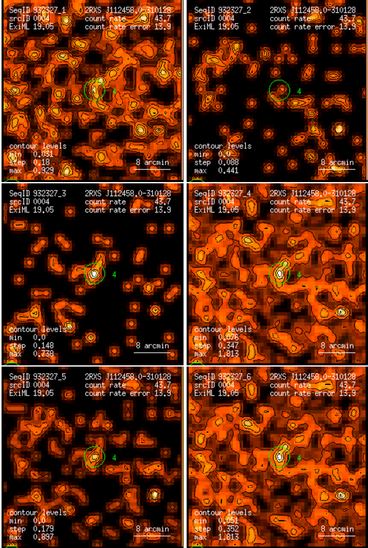
Figure 4: RASS 932327: detection 0004: band rate images, Gaussian filter: (1) PSPC channels 11 – 41, (2) 52 – 90, (3) 91 – 201, (4) 11 – 235, (5) 52 – 201, (6) 11 – 201. Broad band rates in counts/ks. Band rate contour levels in counts/ks/arcmin 2 .
