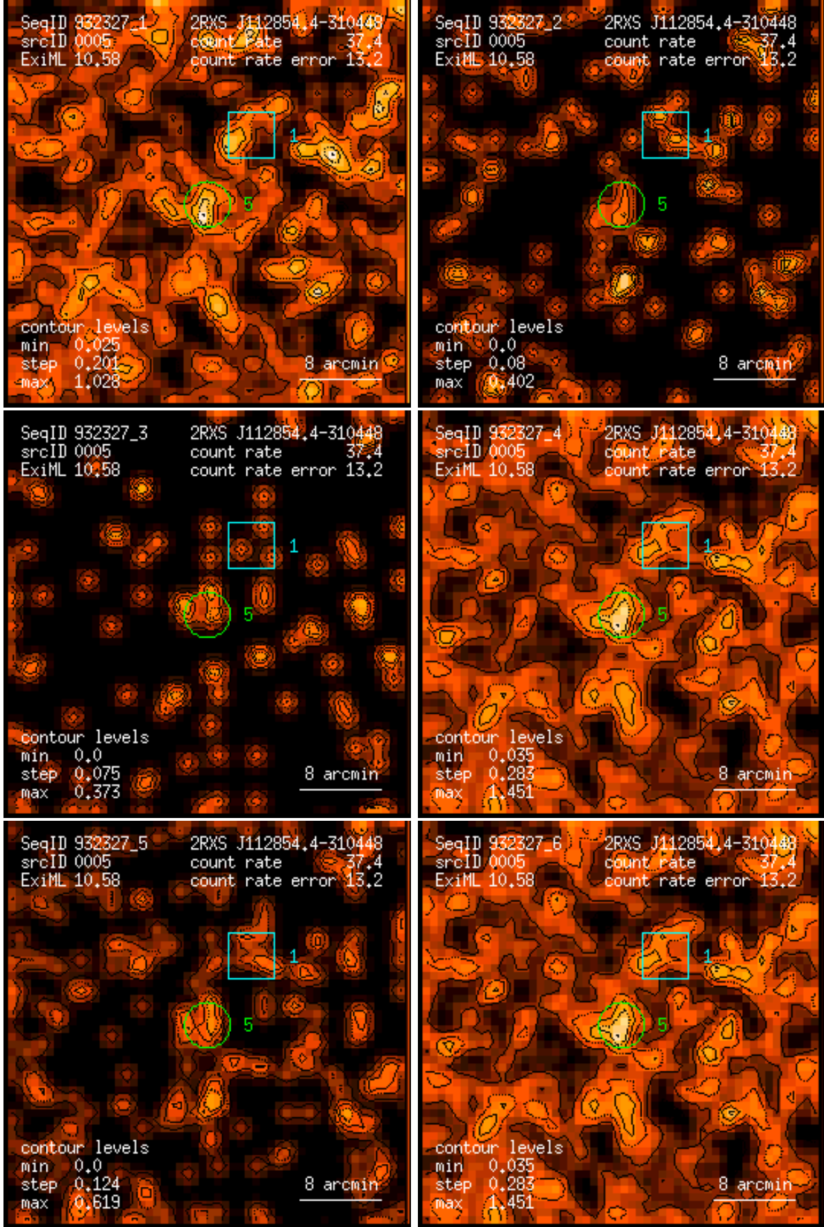
Figure 5: RASS 932327: detection 0005: band rate images, Gaussian filter: (1) PSPC channels 11 – 41, (2) 52 – 90, (3) 91 – 201, (4) 11 – 235, (5) 52 – 201, (6) 11 – 201. Broad band rates in counts/ks. Band rate contour levels in counts/ks/arcmin 2 .
